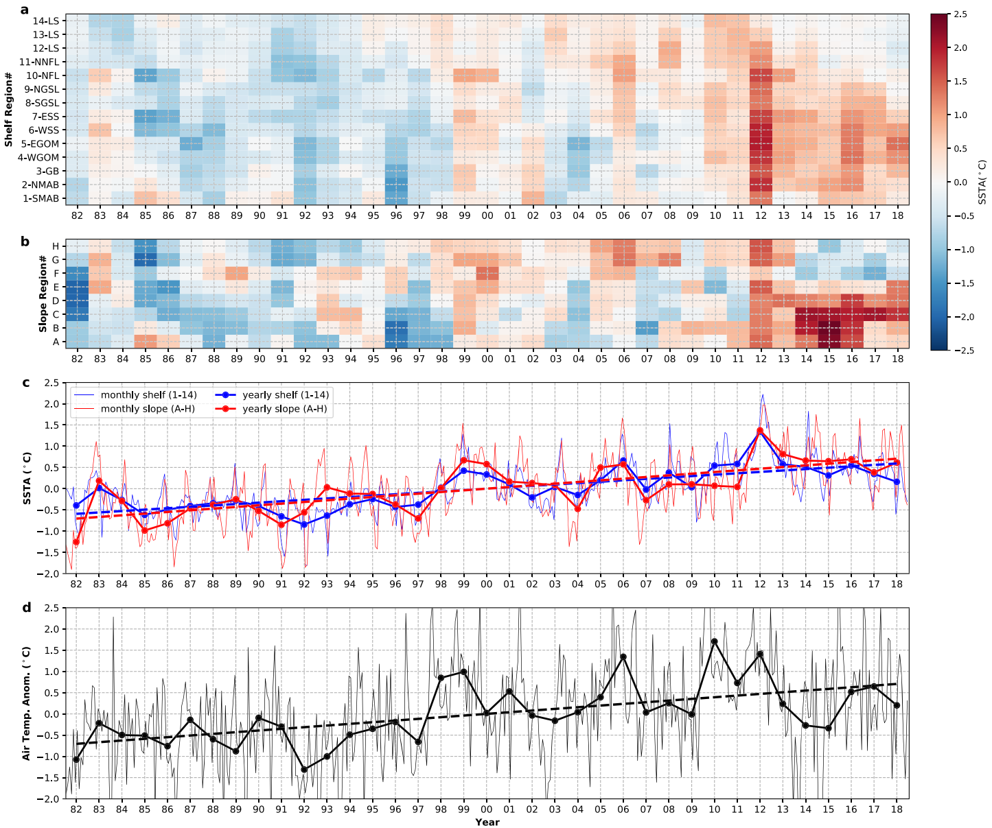
Figure 2. Time series of sea surface temperature anomalies (SSTA) and near-surface air temperature anomalies. (a) Hovmöller diagram of SSTA for the shelf boxes, with x axis representing year and y axis representing regional boxes in a latitudinally increasing order. (b) Same as (a) but for the slope boxes. (c) The meridional means for the shelf boxes 1–14 (blue) and slope boxes A–H (red), in monthly (thin solid lines) and yearly (thick solid lines) means. Linear trends are plotted as the thick dashed lines with corresponding colors. (d) The near-surface air temperature anomalies in monthly (thin solid black line) and yearly (thick solid black line) means based on air temperature observed near the coast over the land (cyan stars on Figure 1). The linear trend is plotted as the thick dashed black line.
