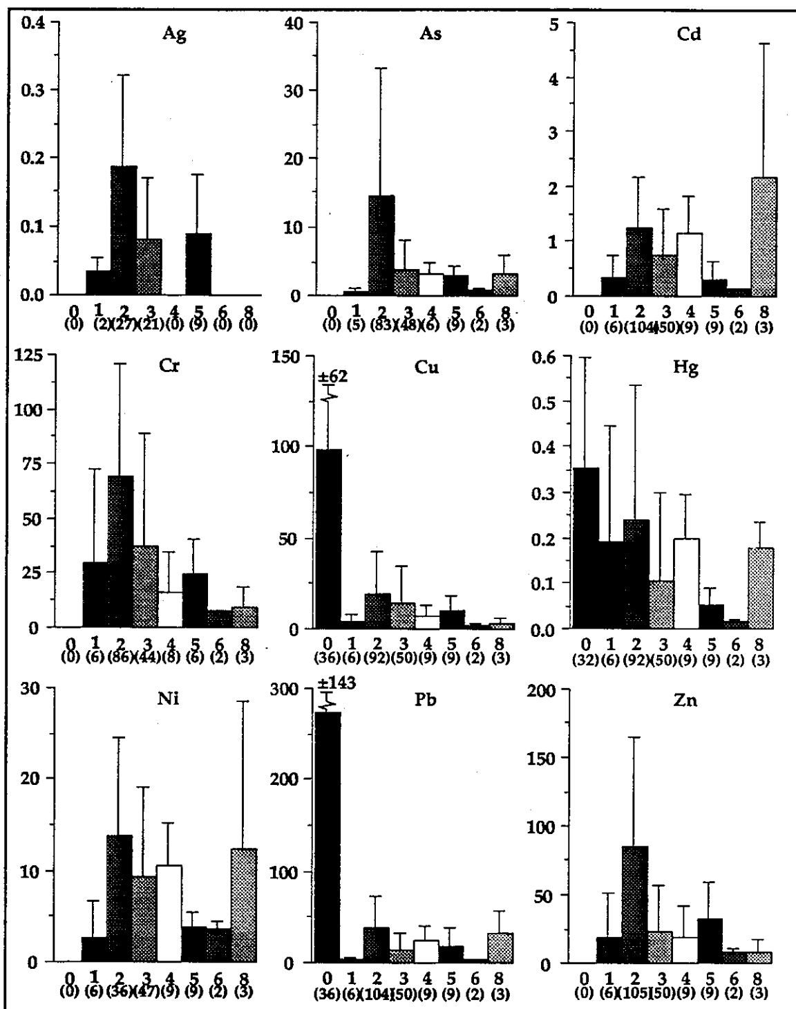
Figure 4. Mean metal concentrations (ppm dw) in the surficial sediments of seven of the eight Tampa Bay subdivisions based on all the available data (numbers in parentheses are sample sizes). Subdivision 0 is the lower Hillsborough River, 1 is Old Tampa Bay, 2 is Hillsborough Bay, 3 is Middle Tampa Bay, 4 is Lower Tampa Bay, 5 is Boca Ciega Bay, 6 is Terra Ceia Bay, and 8 is Gulf of Mexico.
