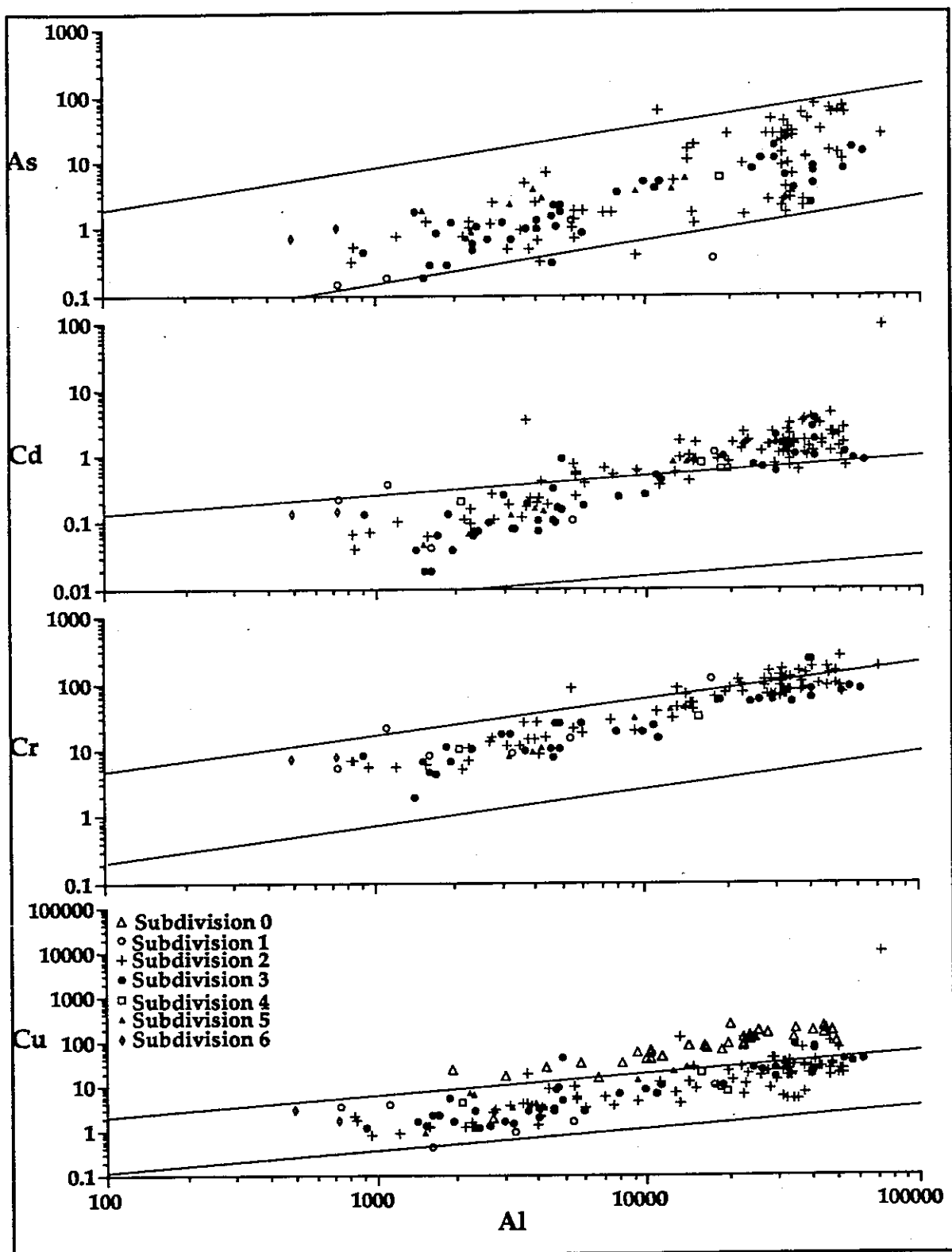
Figure 5. As, Cd, Cr, and Cu concentrations (ppm dw) in the surficial sediments of Tampa Bay from the combined, merged data set plotted against Al concentrations (ppm dw) and the \pm 95\% confidence limits of Schropp et al. (1990).
