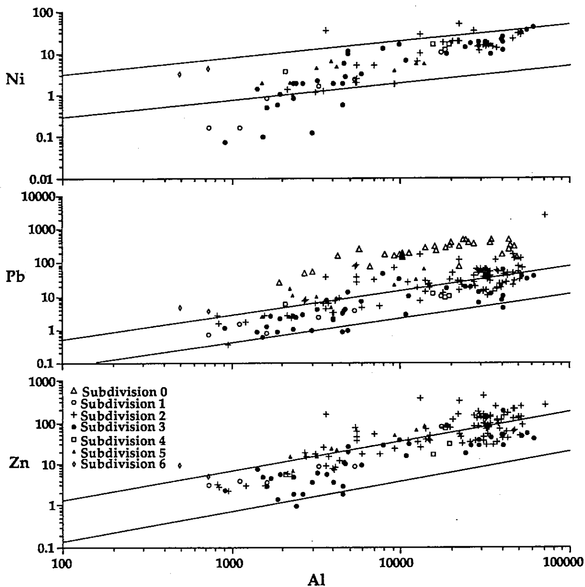
Figure 6. Ni, Pb, and Zn concentrations (ppm dw) in the surficial sediments of Tampa Bay from the combined, merged data set plotted against Al concentrations (ppm dw) and the \pm 95 confidence limits of Schropp et al. (1990).
