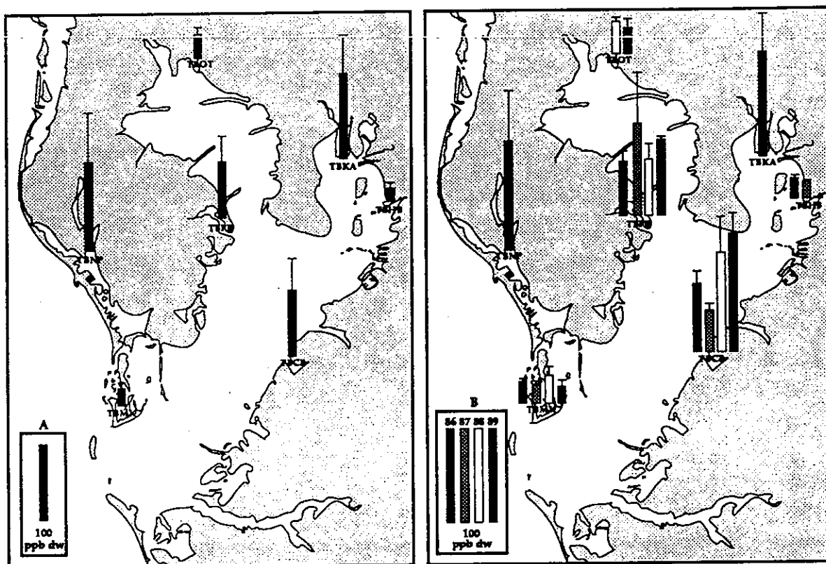
Figure 17. (A) Overall mean and (B) annual mean chlordane concentrations (ppb dw) in oysters from the Tampa Bay area NS&T Program sites for 1986-89 (bars represent one standard deviation).
