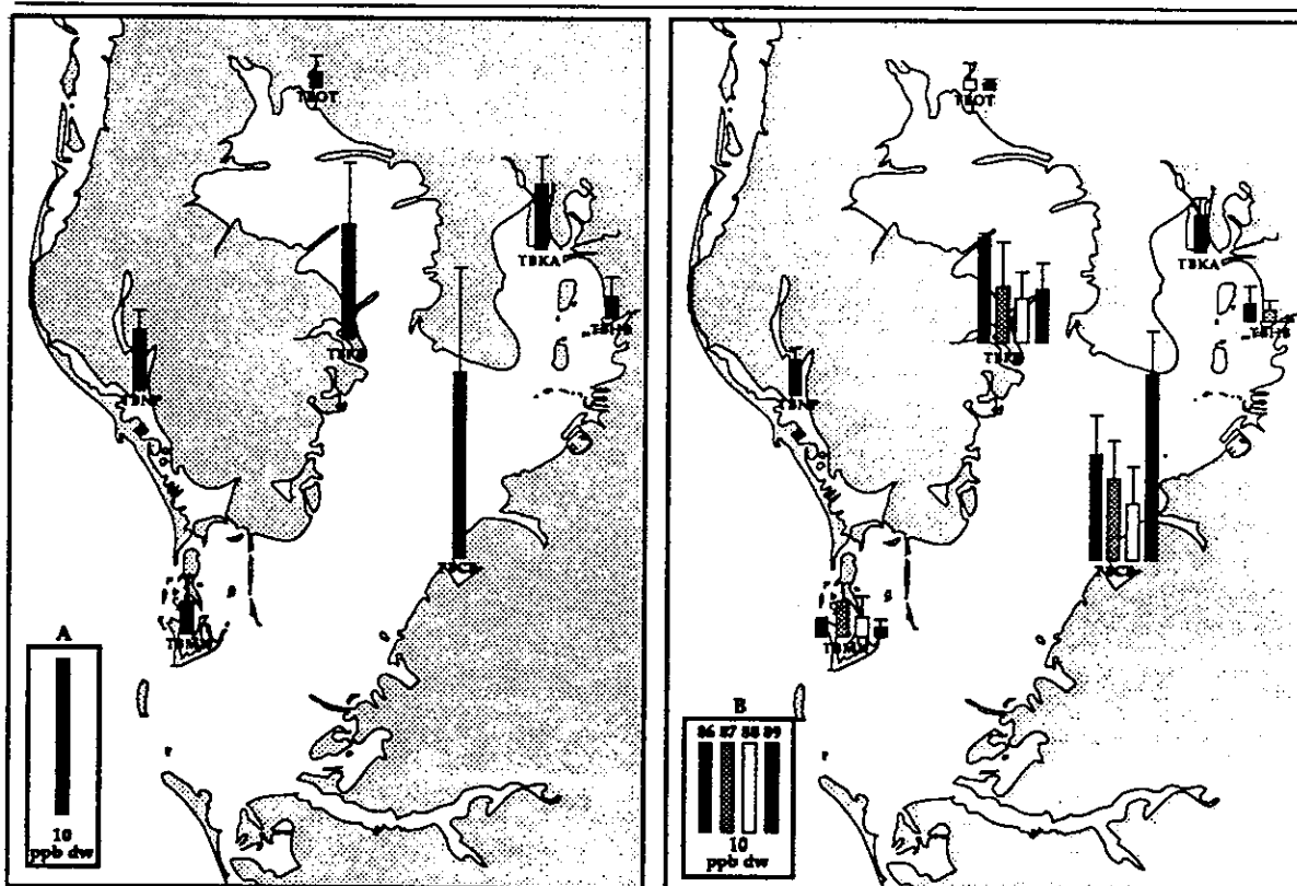
Figure 20. (A) Overall mean and (B) annual mean mirex concentrations (ppb dw) in oysters from the Tampa Bay area NS&T Program sites for 1986-89 (bars represent one standard deviation).
