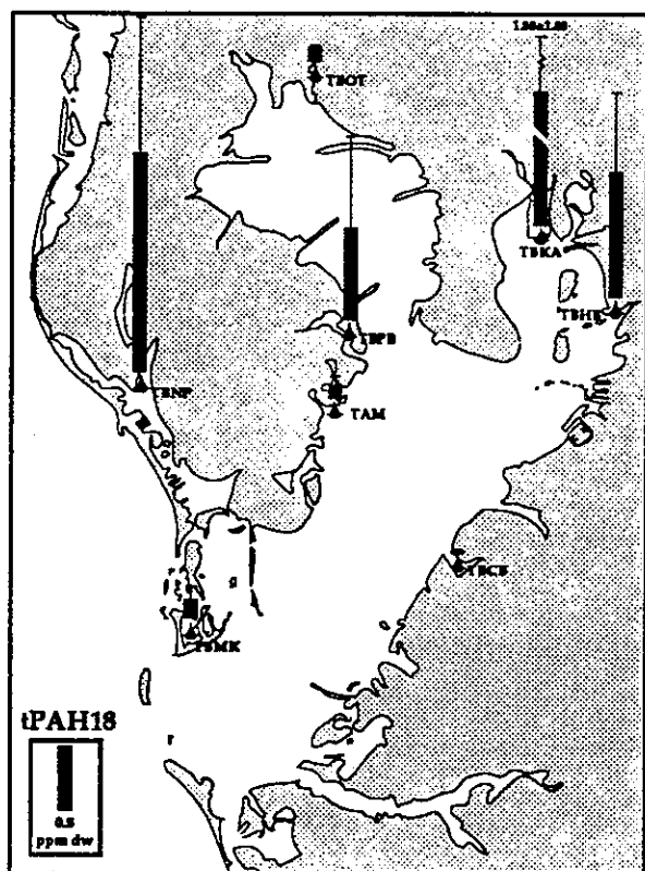
Figure 7. Mean tPAH concentrations (ppm dw) in the surficial sediments collected in 1984-88 at Tampa Bay area NS&T Program sites.
