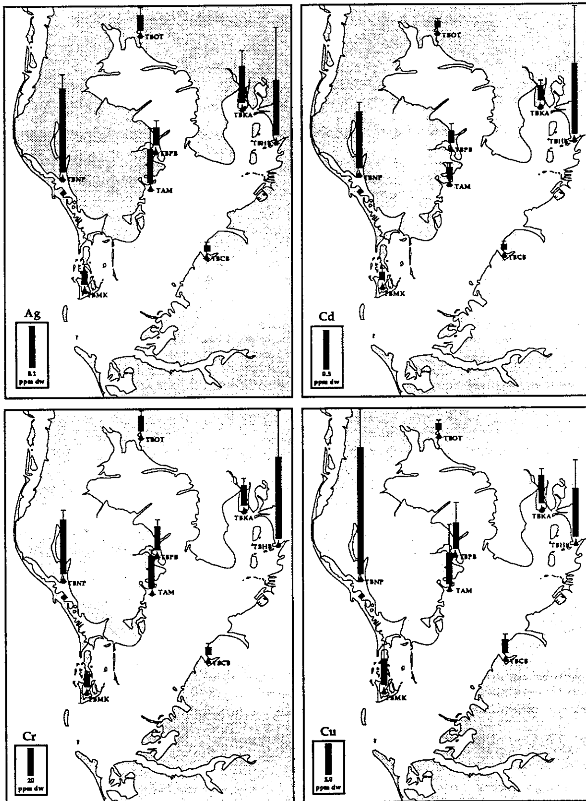
Figure 2. Mean Ag, Cd, Cr, and Cu concentrations (ppm dw) in the surficial sediments NOAA's NS&T Program sites in the Tampa Bay area based on combined data from 1984-88.
