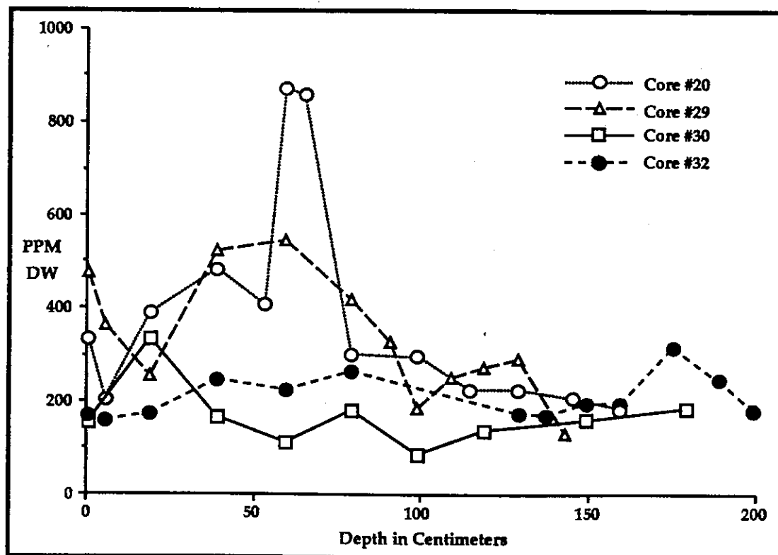
Figure 13. Lead concentrations (ppm dw) in different depth strata below sediment surface in four cores from the lower Hillsborough River (Trefry et al. , 1989).
