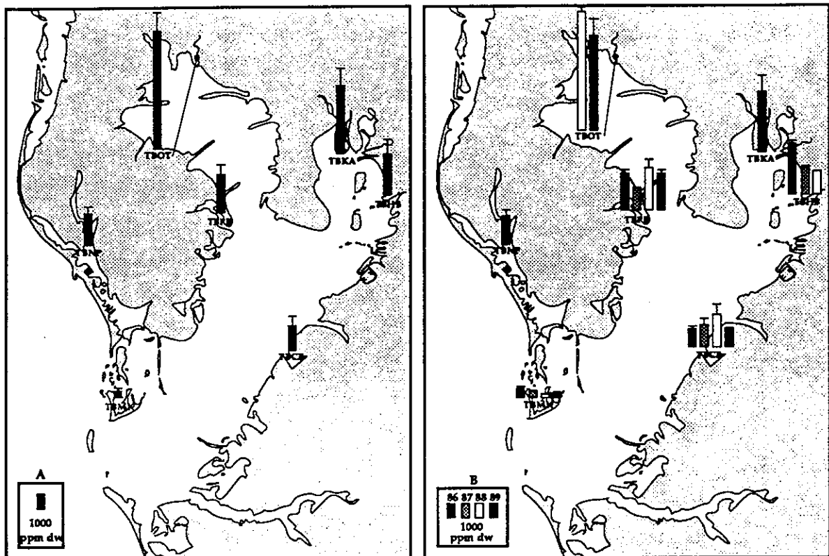
Figure 24. (A) Overall mean and (B) annual mean zinc concentrations (ppm dw) in oysters from the Tampa Bay area NS&T Program sites for 1986-89 (bars represent one standard deviation).
