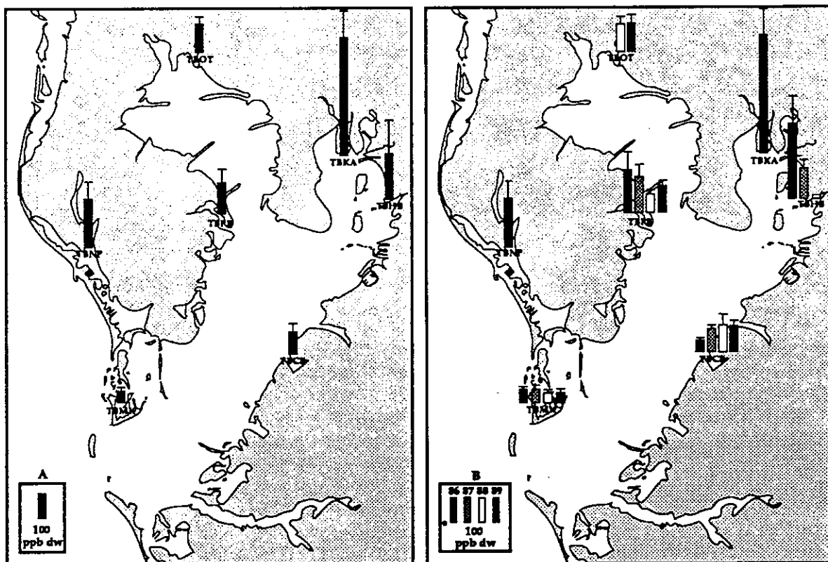
Figure 14. (A) Overall mean and (B) annual mean tPCB concentrations (ppb dw) in oysters from the Tampa Bay area NS&T Program sites for 1986-89 (bars represent one standard deviation).
