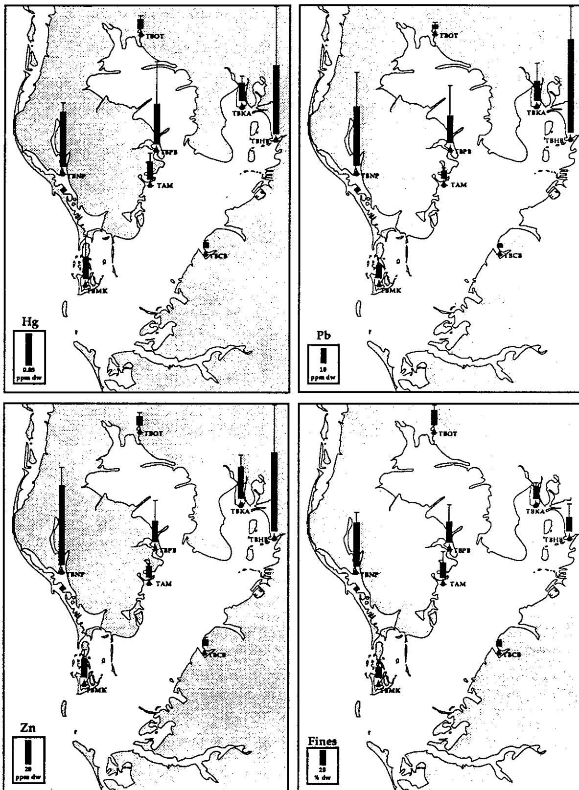
Figure 3. Mean Hg, Pb, and Zn concentrations (ppm dw) and percent fines in the surficial sediments NOAA's NS&T Program sites in the Tampa Bay area based on combined data from 1984-88.
