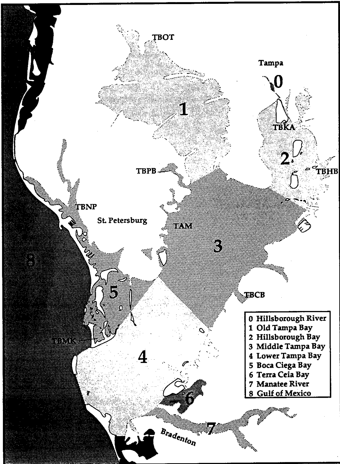
Figure 1. Tampa Bay subdivisions (after Lewis and Whitman, 1985) and locations of NS&T Program sampling sites.
