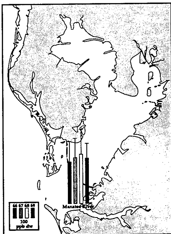
Figure 19. Mean tDDT concentrations (ppb dw) in oysters from the Manatee River site sampled by Butler (1973) during 1966-69 (bars represent one standard deviation).
