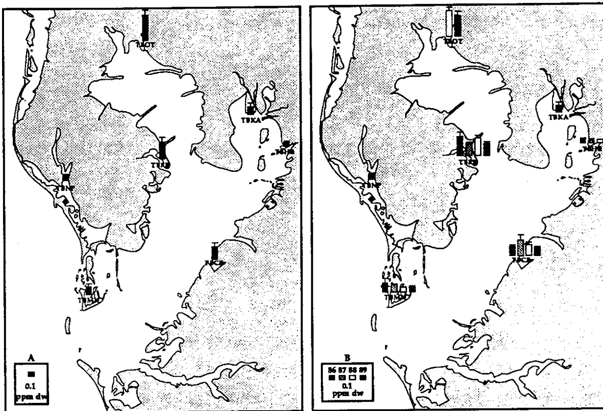
Figure 21. (A) Overall mean and (B) annual mean mercury concentrations (ppm dw) in oysters from the Tampa Bay area NS&T Program sites for 1986-89 (bars represent one standard deviation).
