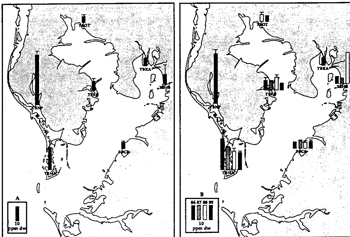
Figure 23. (A) Overall mean and (B) annual mean arsenic concentrations (ppm dw) in oysters from the Tampa Bay area NS&T Program sites for 1986-89 (bars represent one standard deviation).
