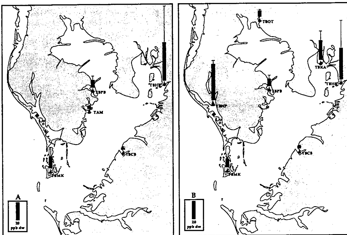
Figure 10. Mean tPCB concentrations (ppb dw) in the surficial sediments of the Tampa Bay area NS&T Program sites based on (A) summed chlorination level concentrations and (B) summed congener concentrations. Excludes single extraneously high sample from TBPB with tPCB concentrations of 230 and 790 ppb dw based on chlorination levels and congener levels, respectively.
