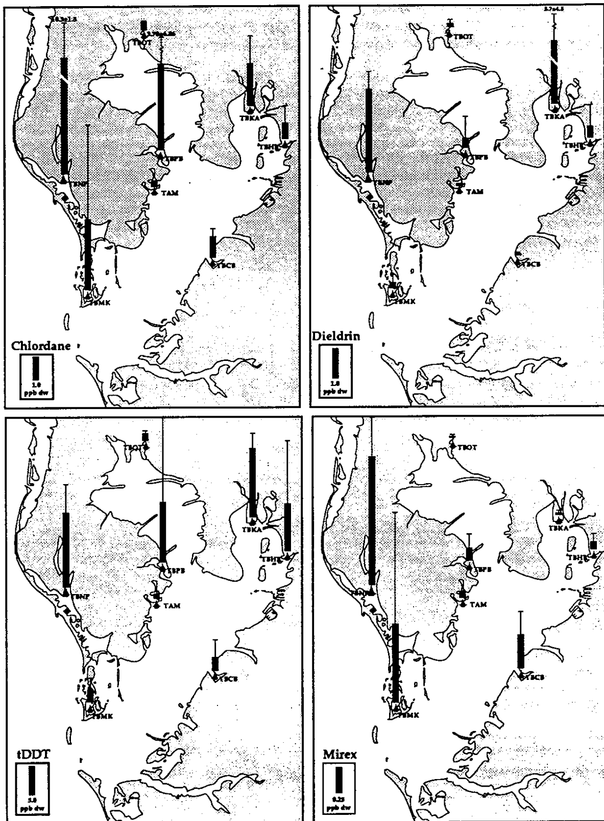
Figure 9. Mean concentrations (ppb dw) and standard deviations of chlordane, dieldrin, tDDT, and mirex in the surficial sediments of the Tampa Bay area NS&T Program sites.
