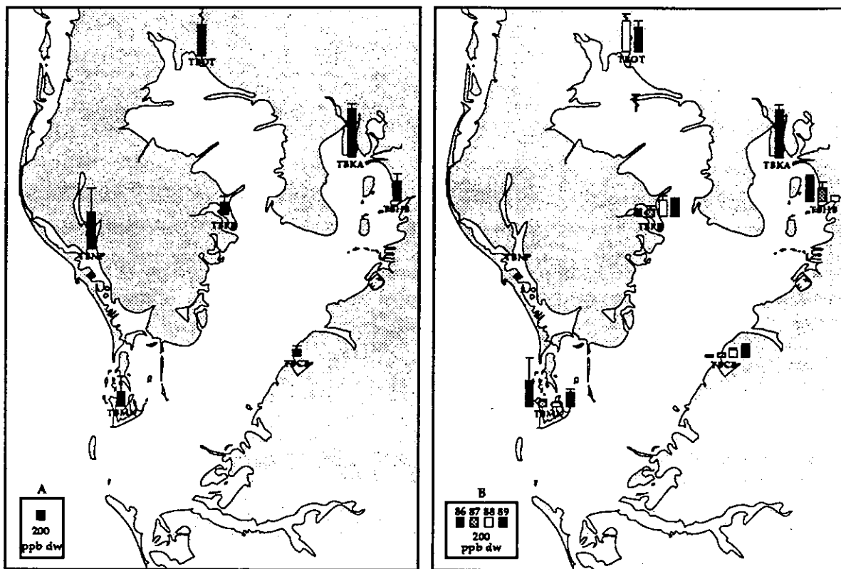
Figure 15. (A) Overall mean and (B) annual mean tPAH concentrations (ppb dw) in oysters from the Tampa Bay area NS&T Program sites for 1986-89 (bars represent one standard deviation).
