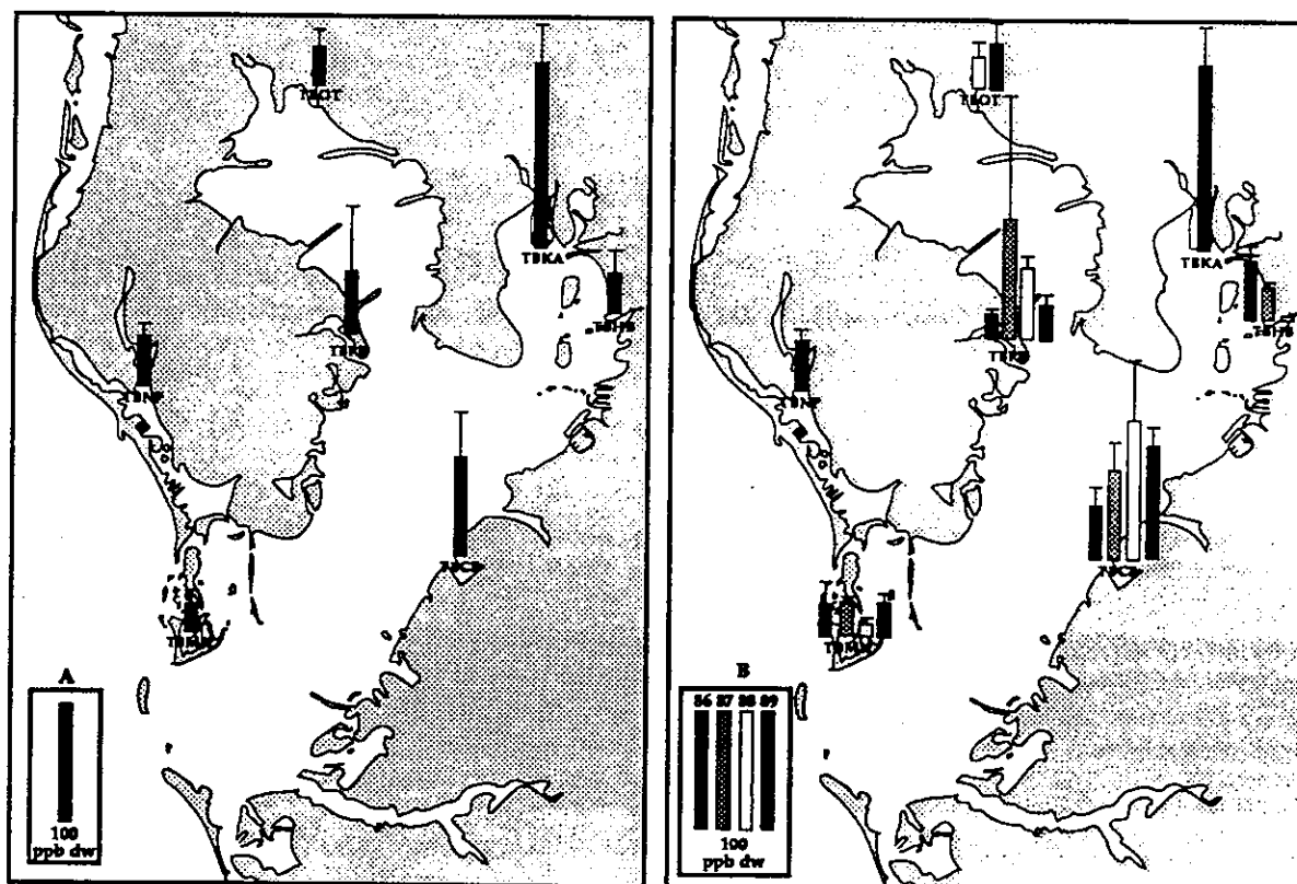
Figure 18. (A) Overall mean and (B) annual mean tDDT concentrations (ppb dw) in oysters from the Tampa Bay area NS&T Program sites for 1986-89 (bars represent one standard deviation).
