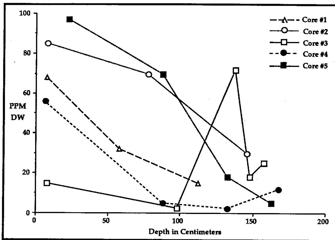
Figure 12. Lead concentrations (ppm dw) in different depth strata below the sediment surface in five cores from the Bradenton Municipal Marina in the lower Manatee River (Wade-Trim, Inc. 1988).
