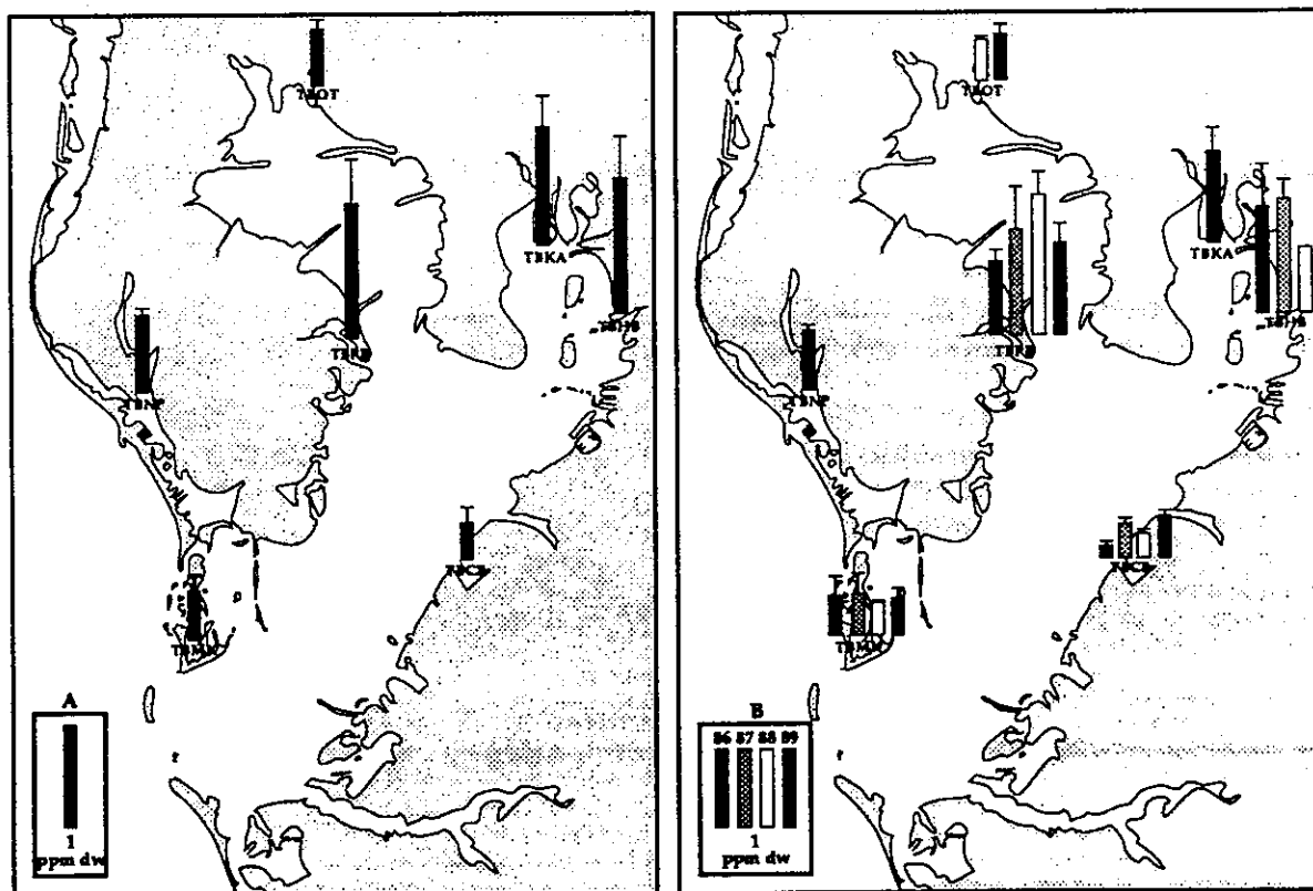
Figure 22. (A) Overall mean and (B) annual mean lead concentrations (ppm dw) in oysters from the Tampa Bay area NS&T Program sites for 1986-89 (bars represent one standard deviation).
