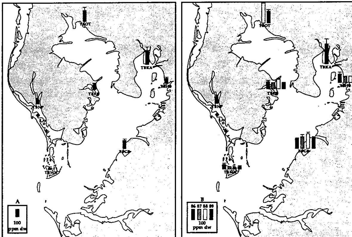
Figure 25 (A) Overall mean and (B) annual mean copper concentrations (ppm dw) in oysters from the Tampa Bay area NS&T Program sites for 1986-89 (bars represent one standard deviation).
