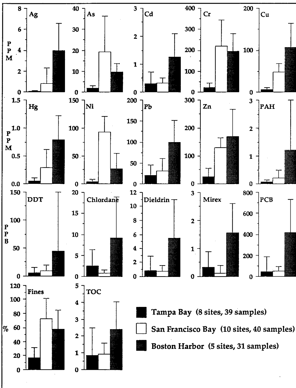
Figure 11. Comparison of the mean concentrations of 15 analytes and 2 normalizers based on the NS&T Program data for Tampa Bay, San Francisco Bay and Boston Harbor (bars represent one standard deviation). The concentrations are in ppm dw for the metals and PAHs, ppb dw for the pesticides and PCBs, and percent for fines and TOC. The PCB means are based solely on the chlorination level data and the Boston Harbor mean excludes one sample which had 51,000 ppb.
