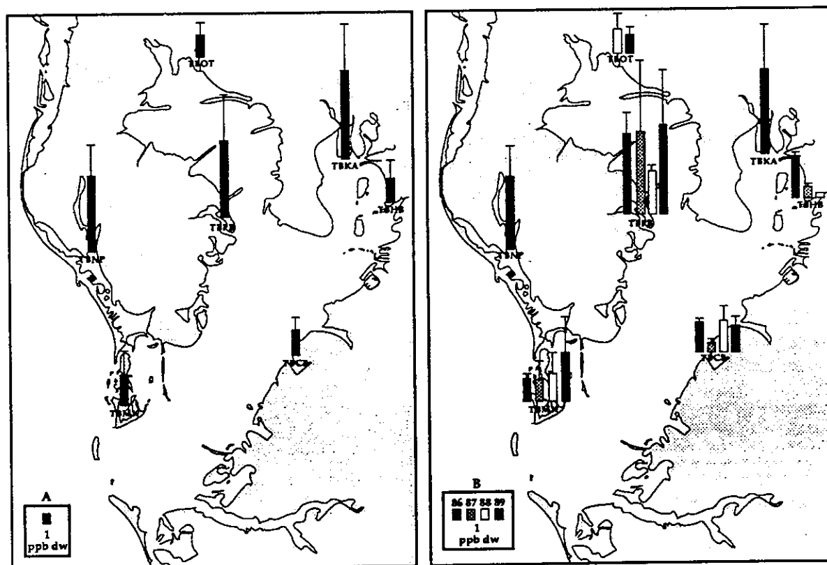
Figure 16. (A) Overall mean and (B) annual mean dieldrin concentrations (ppb dw) in oysters from the Tampa Bay area NS&T Program sites for 1986-89 (bars represent one standard deviation).
