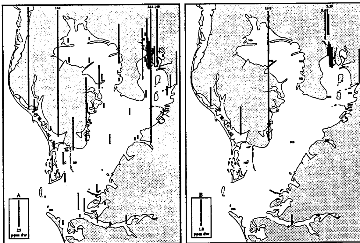
Figure 8. Concentrations (ppm dw) in the surficial sediments of Tampa Bay of the f2 fraction (aromatic and olefinic) hydrocarbons (A) in 1984 and tPAH (B) based on the sum of the concentrations of four families of PAHs (naphthalenes, phenanthrenes, pyrenes, benz(a)anthracenes) in 1984-85 (from Doyle et al. , 1985).
