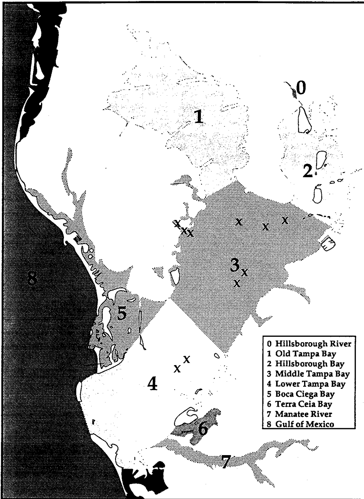
Figure 26. Sediment toxicity sampling locations in Tampa Bay (from Environmental Science and Engineering, 1979; Jones, Edmunds and Associates, 1979, 1980).
