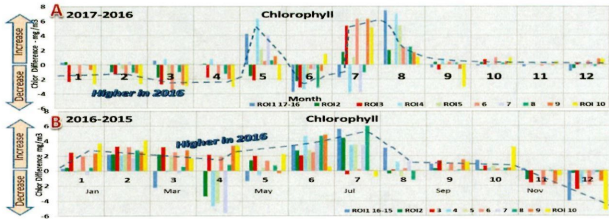
Figure 8 –Yearly differences for each month in the chlorophyll-a seasonal cycle: (A) 2017 minus 2016 and (B) 2016 minus 2015 for each ROI. Scales: (A) Positive Chlorophyll-a in 2017 is higher than 2016 (B) Positive Chlorophyll-a in 2016 is higher than 2015.
