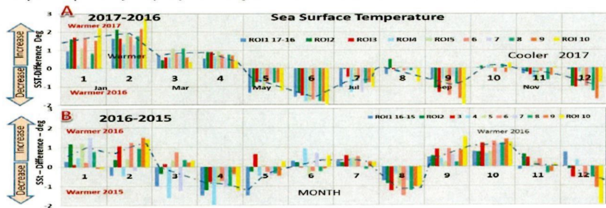
Figure 10: Yearly differences in the Sea Surface Temperature for the monthly seasonal cycle at the 10 ROI locations across the Shelf: (A) 2017 minus 2016 and (B) 2016-2015 for each of the Shelf. Warmer months have positive increased yearly SST in A) 2017 and B) 2016. Negative SST is monthly cooling from previous year
