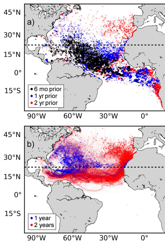
Fig. 4. Global HYCOM backtracking model results. (a) Locations of 30,000 synthetic particles initially released between April and June 2011 at random locations and at 5-day intervals throughout the Caribbean Sea after being backtracked for 6 months (black dots), 1 year (blue dots), and 2 years (red dots). The dashed line indicates latitude 23°N, the southern boundary of “North Atlantic origin” used by Wang et al. (2019a). Synthetic particles were tracked through HYCOM surface currents with a 1% windage factor applied from 10 m NCEP winds, following the methods described in detail in Putman et al. (2018) and adopted by Wang et al. (2019a). (b) Trajectories of only those particles that were backtracked from the Caribbean Sea to the North Atlantic (> 23°N) within 1 year (blue) or 2 years (red). Tracks indicate two primary routes based on transport duration: a shorter western route through the Greater Antilles which impacted the northeastern Caribbean Sea (blue), and a longer eastern route through the tropical Atlantic and Lesser Antilles that impacted a wider area across the Caribbean Sea (red).
