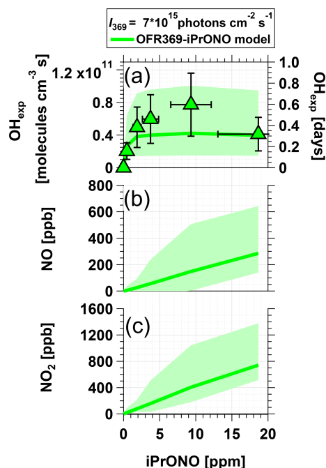
Figure 3. Measured and modeled (a) OH exposure, (b) NO mixing ratio, and (c) NO 2 mixing ratio values obtained using OFR369-i(iPrONO) at I_{369} = 7 \times 10^{15} photons cm -2 s -1 as a function of the iPrONO mixing ratio. Error bars for measurements represent \pm 50 % uncertainty in OH exp and estimated \pm 30 % uncertainty in the iPrONO mixing ratio values.
