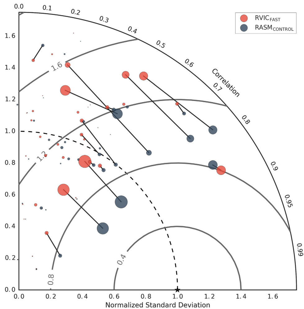
Figure 6. Taylor diagram showing performance of the RVIC model RASM_{CONTROL} (blue) and RVIC_{FAST} (red) for 51 of the largest rivers in the RASM domain. The reference data set used as the comparison is D2009 . Contours, shown in gray denote constant centered root-mean-squared-differences. The lines connecting points (only shown for rivers with an annual mean flow greater than 1000 \text{ m}^3/\text{s} ) represent the change in performance from RVIC_{FAST} to RASM_{CONTROL} .
