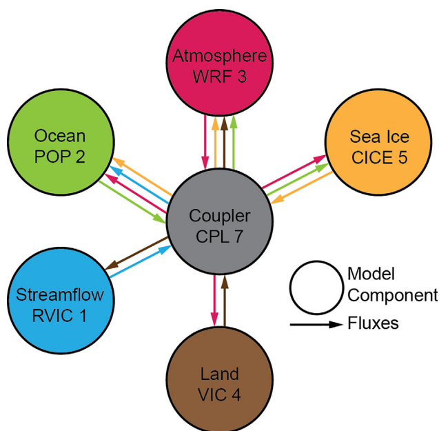
Figure 1. Coupling schematic for the Regional Arctic System Model. Circles represent model components (e.g., RVIC) and arrows between circles represent flux and state variables shared between components (e.g., streamflow). The colors of the arrows reflect the source of the fluxes and state variables.
