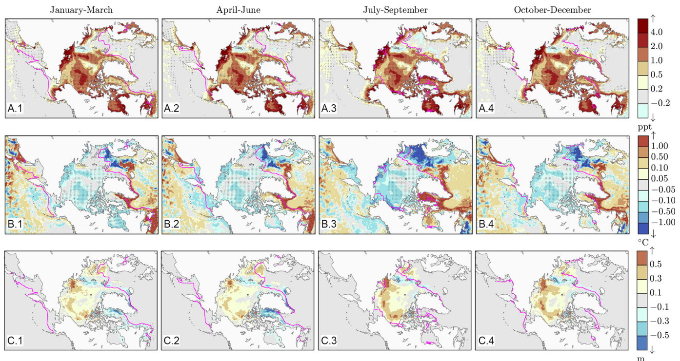
Figure 9. Seasonal difference ( RASM_{NOROF} - RASM_{CONTROL} ) in (top) mean sea surface salinity, (middle) sea surface temperature, and (bottom) sea ice thickness (2000–2009). Stippling denotes differences that are statistically significant at the 95% confidence interval. The magenta contour represents the observed 15% sea ice concentration contour.
