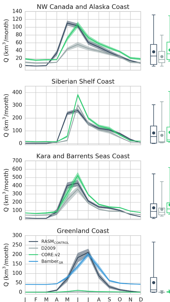
Figure 7. (left) Annual cycle of coastal streamflow fluxes for the four masks shown in Figure 2 comparing RASM_{CONTROL} (dark blue), D2009 (gray), CORE.v2 (green), and Bamber GR (light blue, Greenland only). Solid lines represent the 1991–1999 mean and the shading denotes the interannual variability. (right) Box and whisker from the monthly time series. Whiskers represent the full data range, circles represent the mean, horizontal lines represent the median, and the box represents the first and third quartiles.
