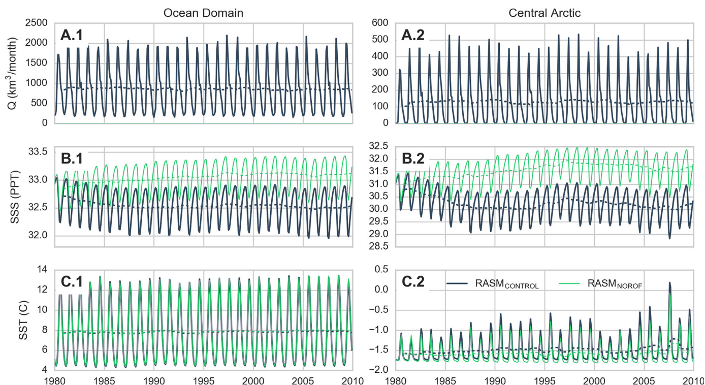
Figure 8. Monthly time series (1980–2009) of (left) domain-wide and (right) central Arctic (top) streamflow ( RASM_{CONTROL} only), (middle) mean SSS, and (bottom) SST for the RASM_{CONTROL} (blue) and RASM_{NOROF} (green). The dashed lines show a 12 month running mean.
