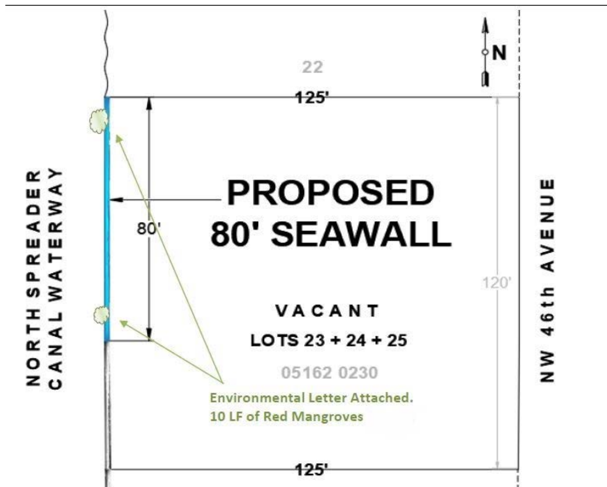
Figure 4. The Gould Seawall project site at 2742 Northwest 46 th Avenue, Cape Coral, Lee County, Florida, showing 80 lin ft of unconsolidated shoreline and the location of red mangroves to be removed. Image supplied by USACE.
