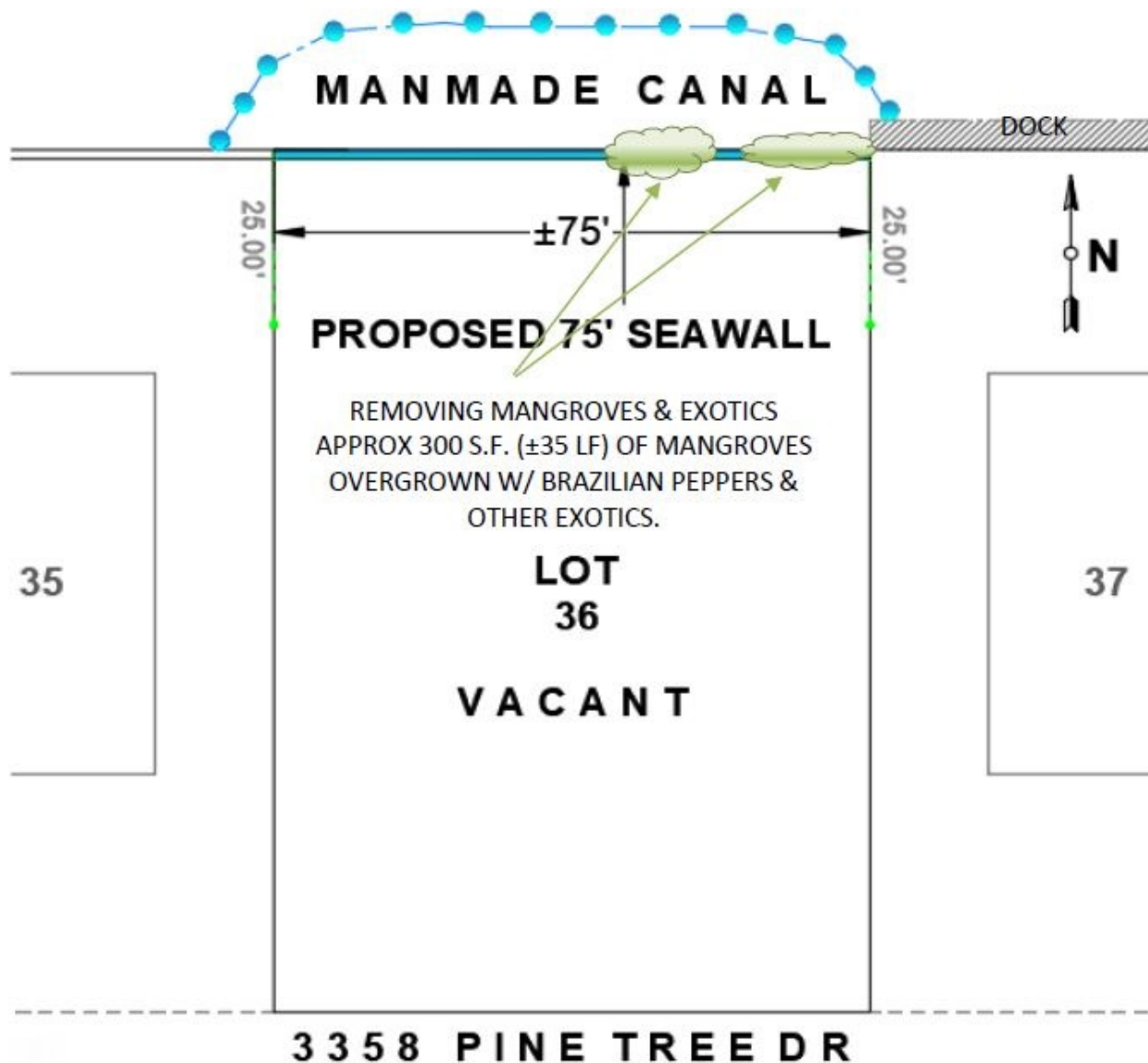
Figure 2. The Cwalina Seawall project site at 3358 Pine Tree Drive, Saint James City, Lee County, Florida, showing 75 linear feet of unconsolidated shoreline and the location of red mangroves to be removed. Image supplied by USACE.
