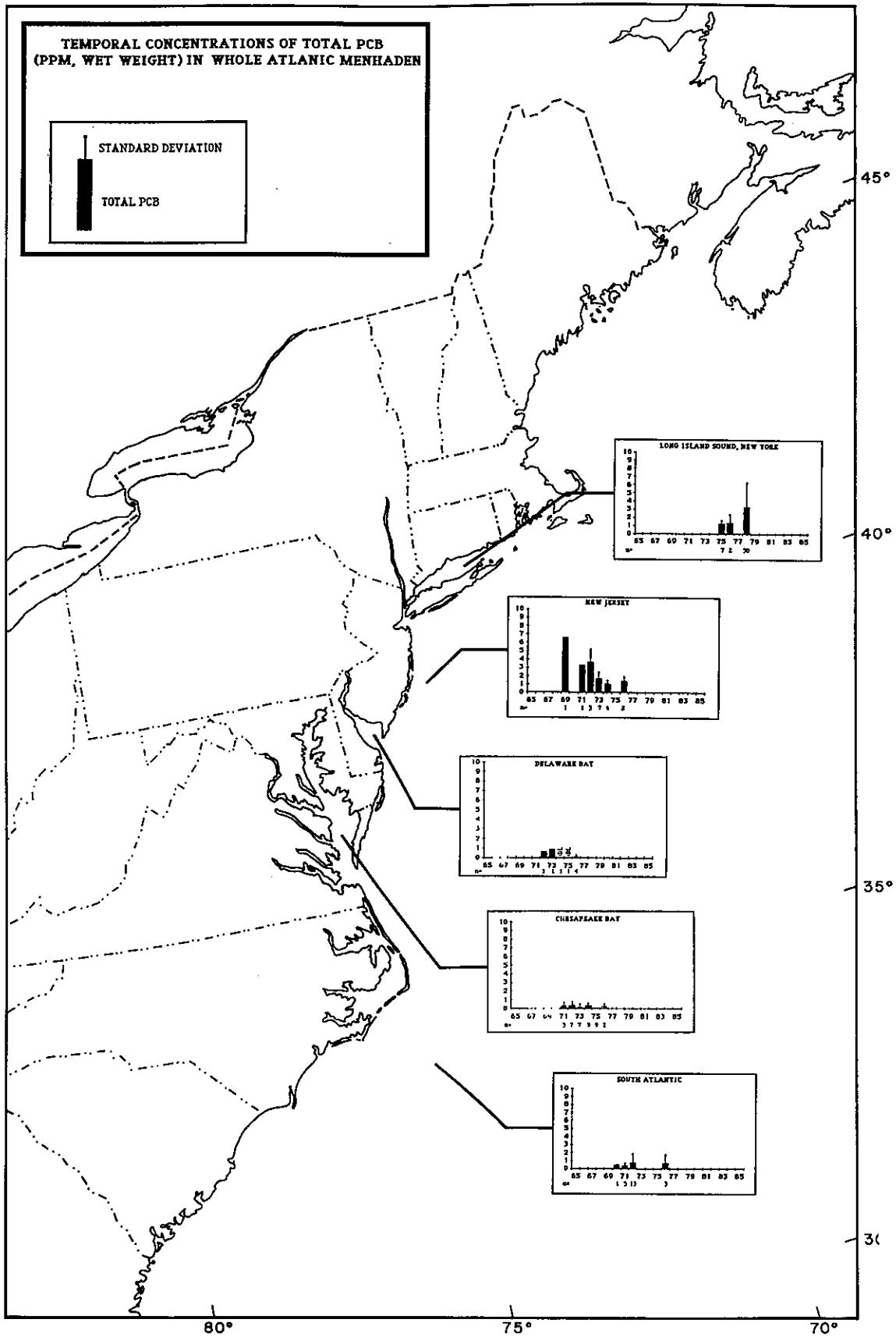
Figure 7.1. Annual variations of average tPCBs (Aroclor) in whole Atlantic menhaden from five Atlantic Coast areas 1969-78. Based on data from sources cited in text.
