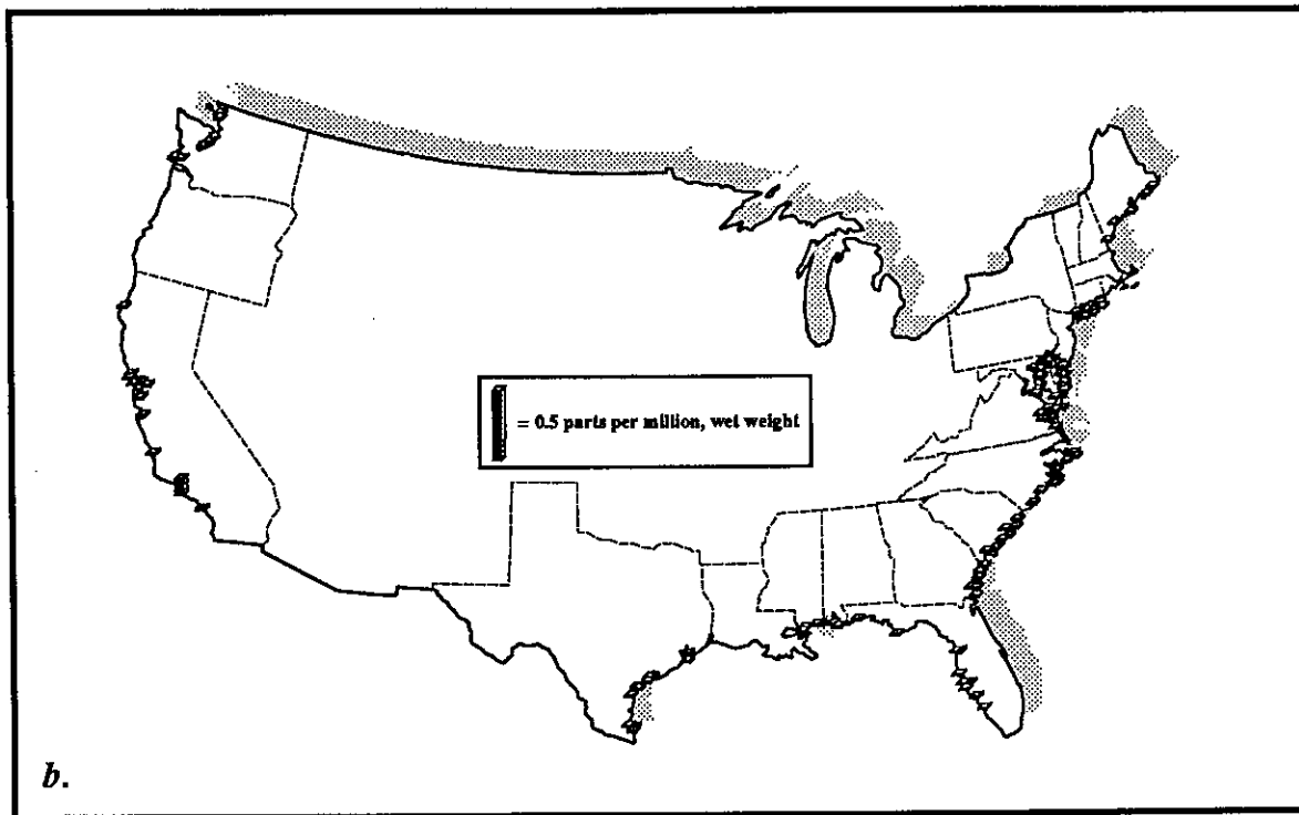
Figure 4.7. Total DDT in estuarine bivalves from 89 estuaries sampled in (a) 1965-72; and (b) 1977. Computed from original data supporting Butler (1973), and Butler et al. (1978). Bar represents mean of (generally) two composite values at each site.
