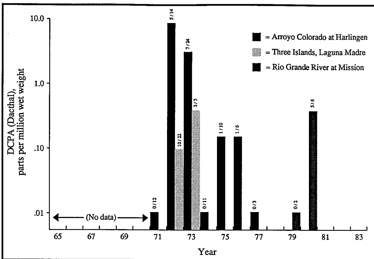
Figure 5.10. Trends in maximum concentrations and frequencies of occurrence (fraction) of DCPA (dacthal) in fishes of the Arroyo Colorado, Rio Grande River, and southern Laguna Madre, Texas, 1971-80. Based on applicable data in references cited in Figure 5.6. Note log scale.
