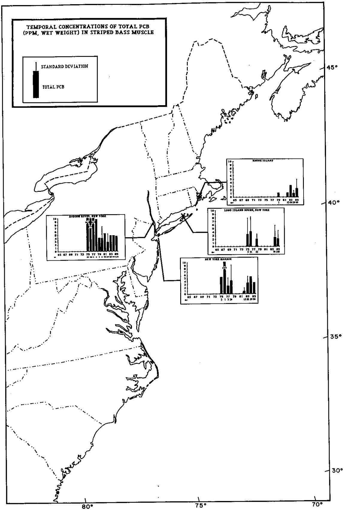
Figure 7.6. Annual variations of average tPCB (Aroclors) in muscle of striped bass from four Atlantic Coast sites or regions, 1976-85. Based on data from various sources cited in text.
