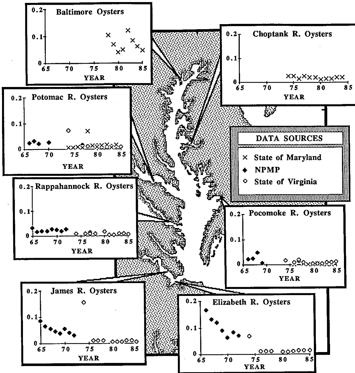
Figure 5.3. Annual variations of tDDT in oysters from seven Chesapeake Bay estuarine segments, 1965-85. Mean concentrations computed from data in Butler, 1973; Butler et al., 1978; and in original data provided by the States of Maryland and Virginia.
