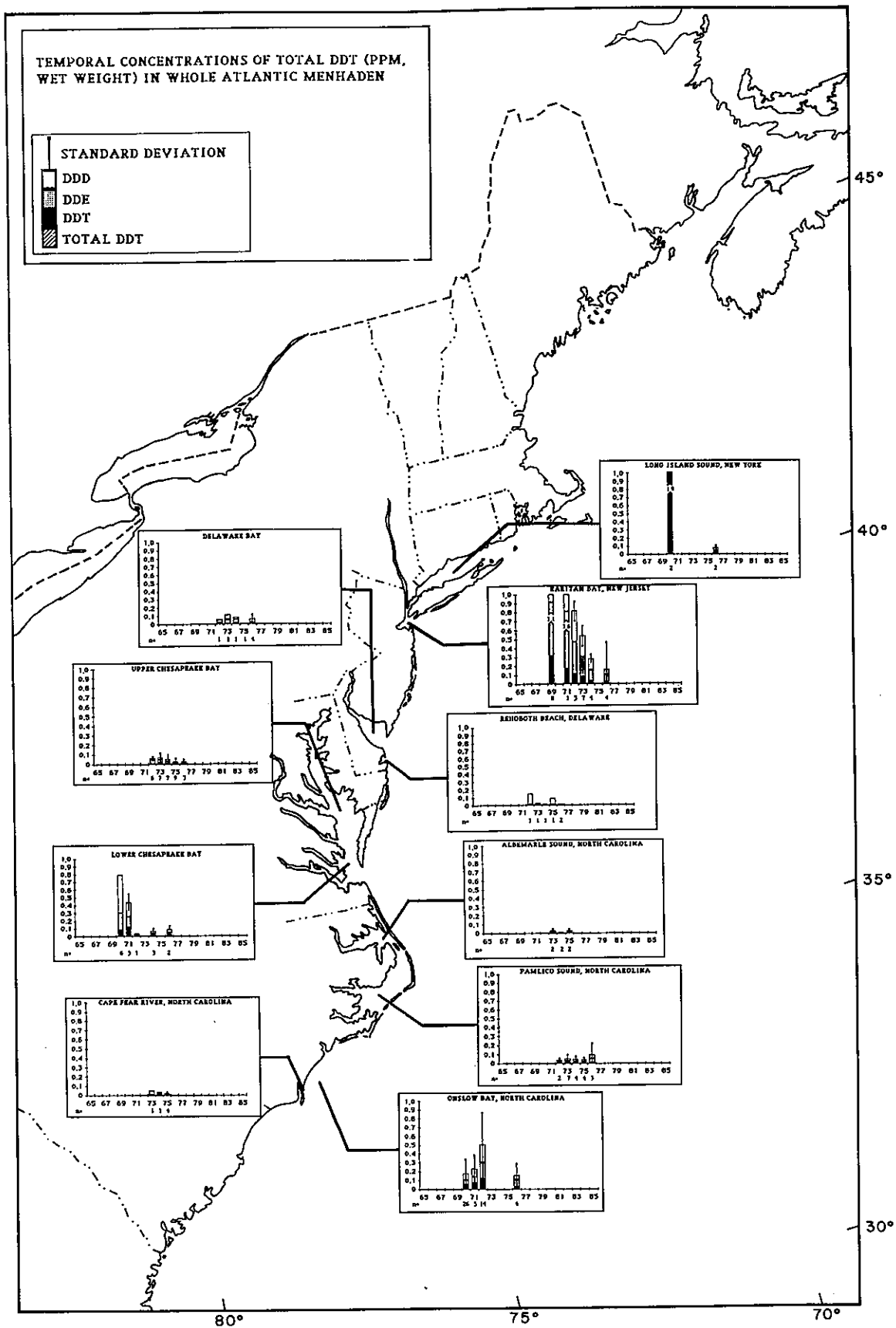
Figure 7.3. Annual variations of average tDDT in whole Atlantic menhaden from 10 collecting or reduction plant sites along the Atlantic Coast, 1969-76. Based principally on original data supporting Stout et al., 1981 and Butler and Schutzmann, 1978. See text for more details.
