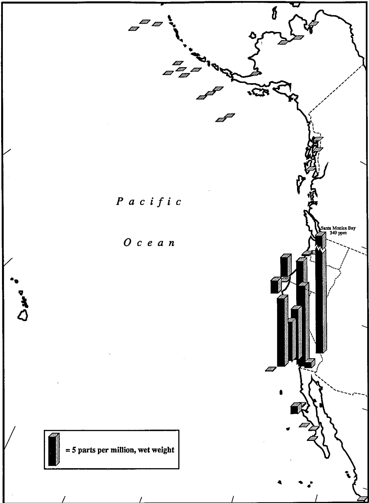
Figure 4.14. Total DDT in livers of fish from various sites in the northeast Pacific Ocean during 1970. Bar represents given value and mean. Species vary among sites. From Duke and Wilson (1978). Compare to Figures 4.12 and 4.13.
