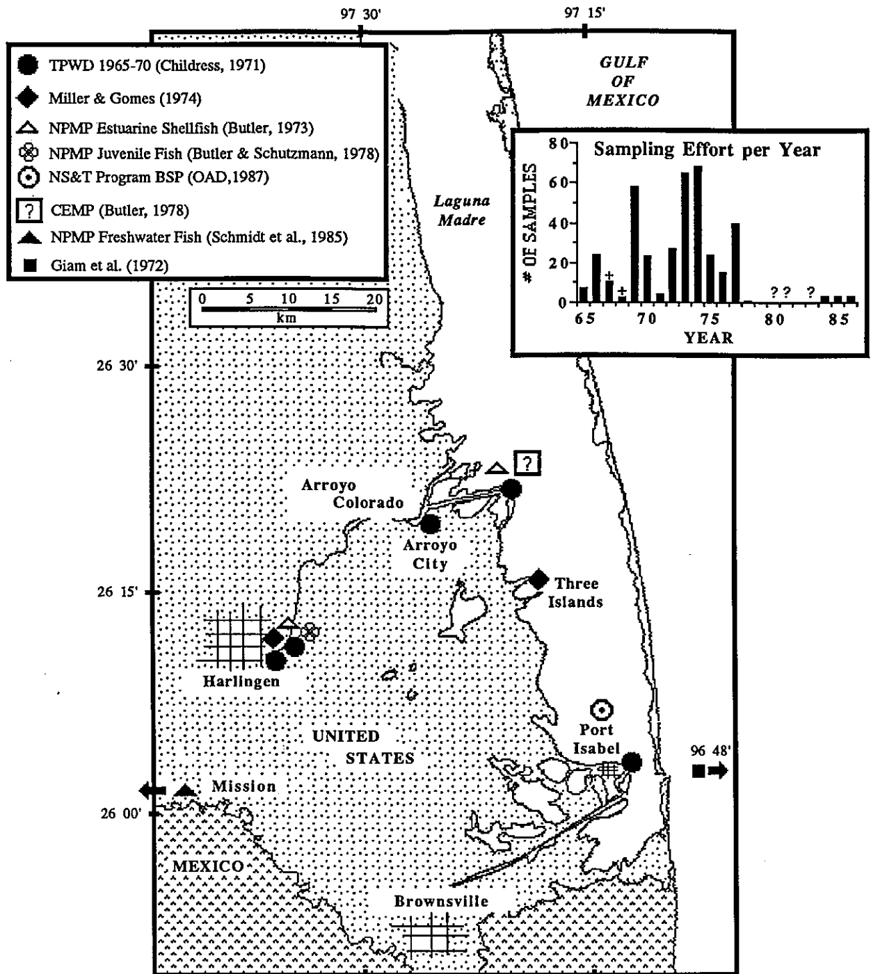
Figure 5.6. Overview of pesticide and PCB monitoring activity in the Arroyo Colorado and Laguna Madre area, Texas, 1965-86.
