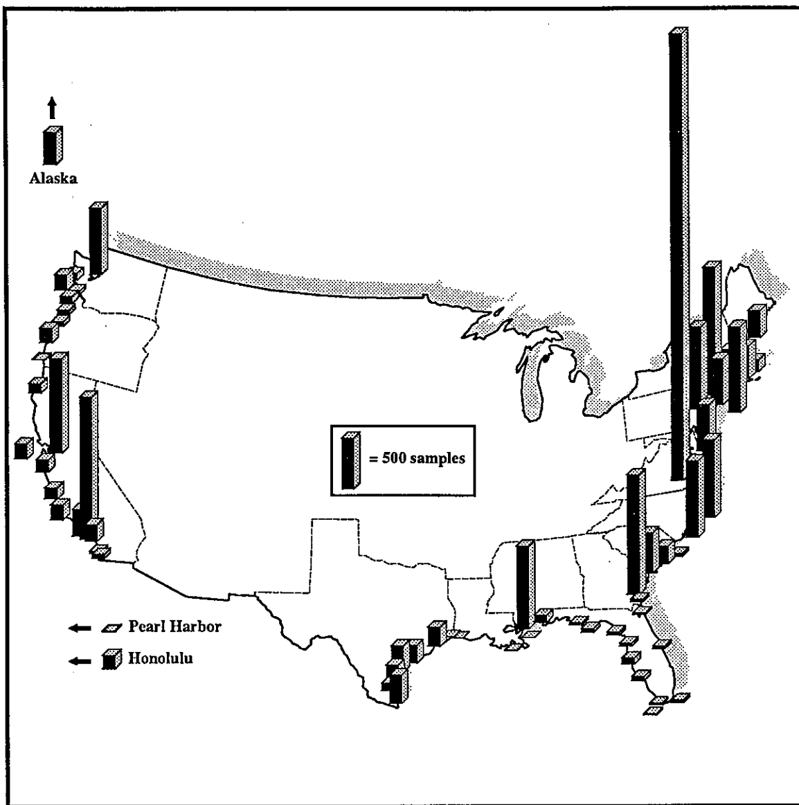
Figure 3.1. Geographic distribution of numbers of samples analyzed for PCBs and/or chlorinated pesticides, 1940 to 1985. Based on data residing in OAD database system, June 1987.
