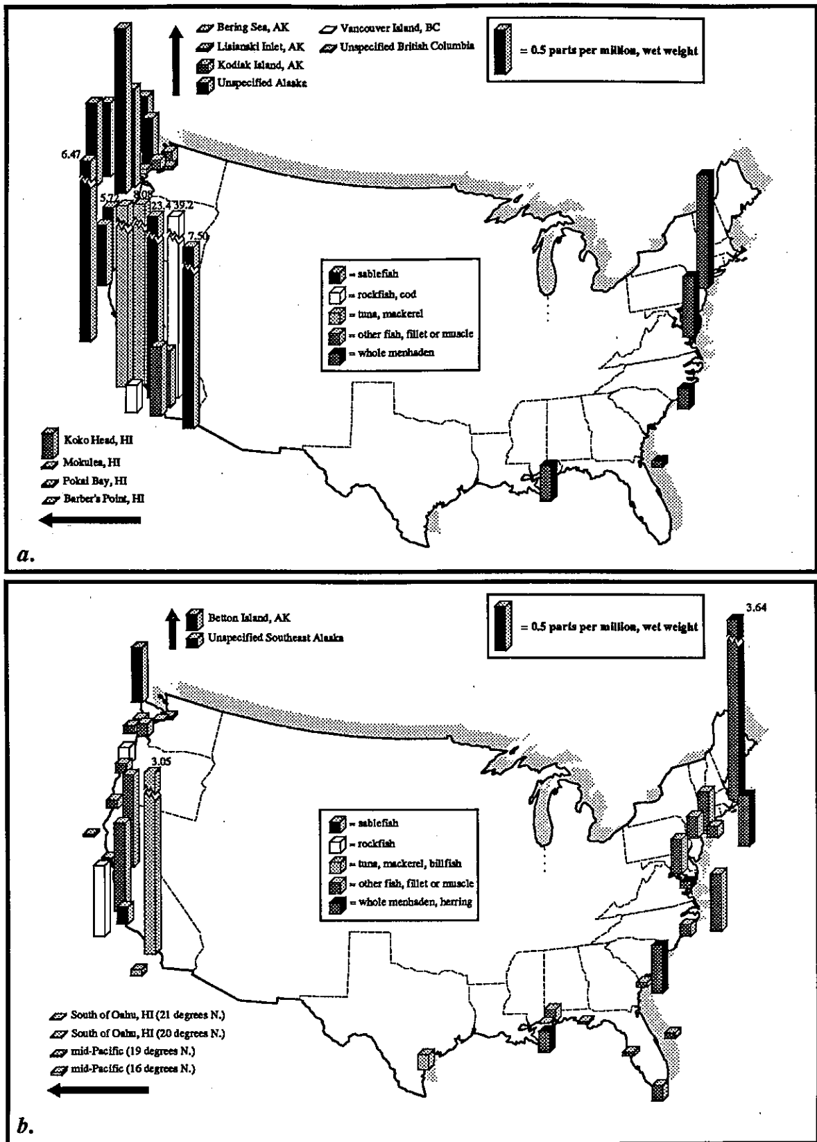
Figure 4.10. Total DDT in fillets (muscle of many species) or whole fish (menhaden) for (a) 1969-71, and (b) 1972-75. Bar represents given mean or mean computed from original data. Compiled from original data supporting Stout (1980); Stout and Beezhold (1981); and Stout et al. (1981).
