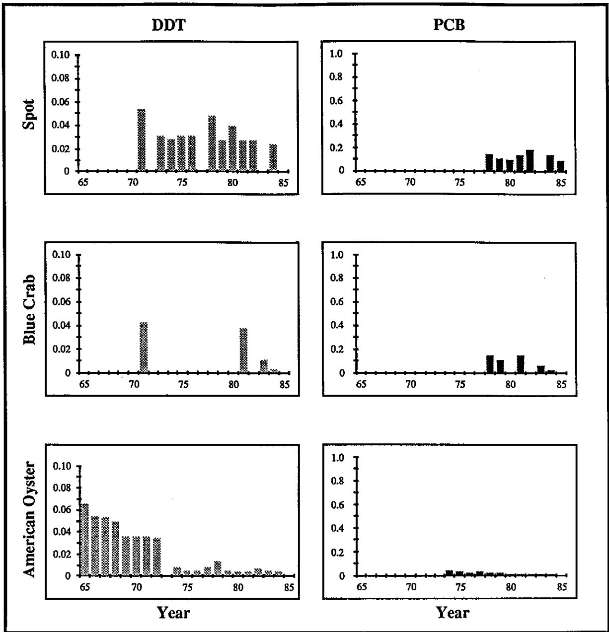
Figure 5.4. Comparison of annual variations of DDT and PCB contamination in all samples of spot, blue crabs, and oysters from the Chesapeake Bay, 1965-85. Based on data as cited previously (Figures 5.2 and 5.3). Units in parts per million, wet weight.
