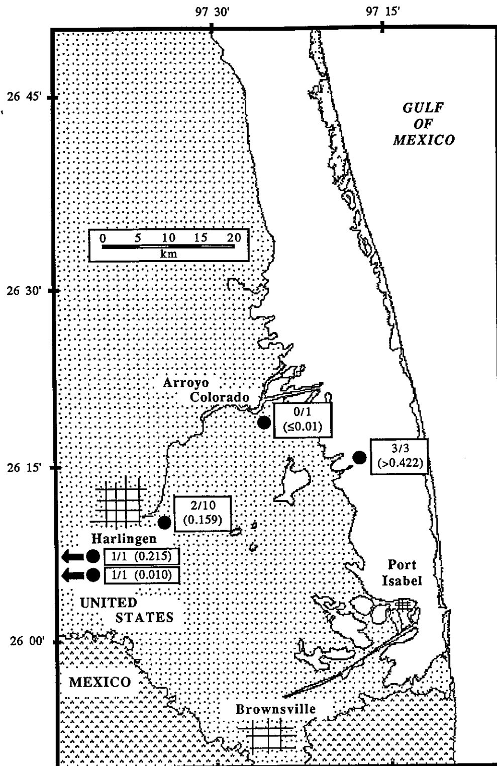
Figure 5.9. Frequency of occurrence (fraction) and maximum concentrations (ppm ww) of the herbicide DCPA (dacthal) in marine and freshwater fish of the Arroyo Colorado system, Texas, 1973. From data in Miller and Gomes (1974) and original data supporting Butler (1978).
