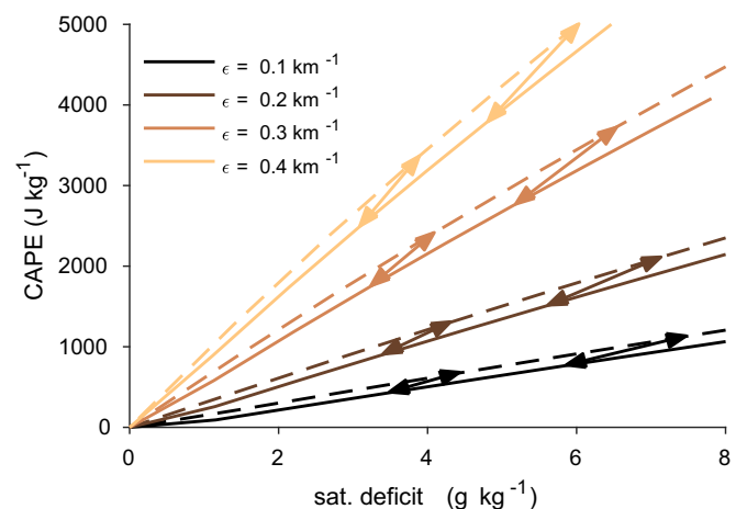
Fig. 4. CAPE as a function of lower-tropospheric saturation deficit q_{\text{def}} calculated using the zero-buoyancy plume model. Calculations are performed with a surface relative humidity of 80% and surface temperatures of 300 K (solid) and 303 K (dashed) for values of the environmental relative humidity in the free troposphere varying between 20% and 100% and entrainment rates \epsilon as given in the legend. Arrows connect solutions with the same relative humidity for different surface temperatures.
