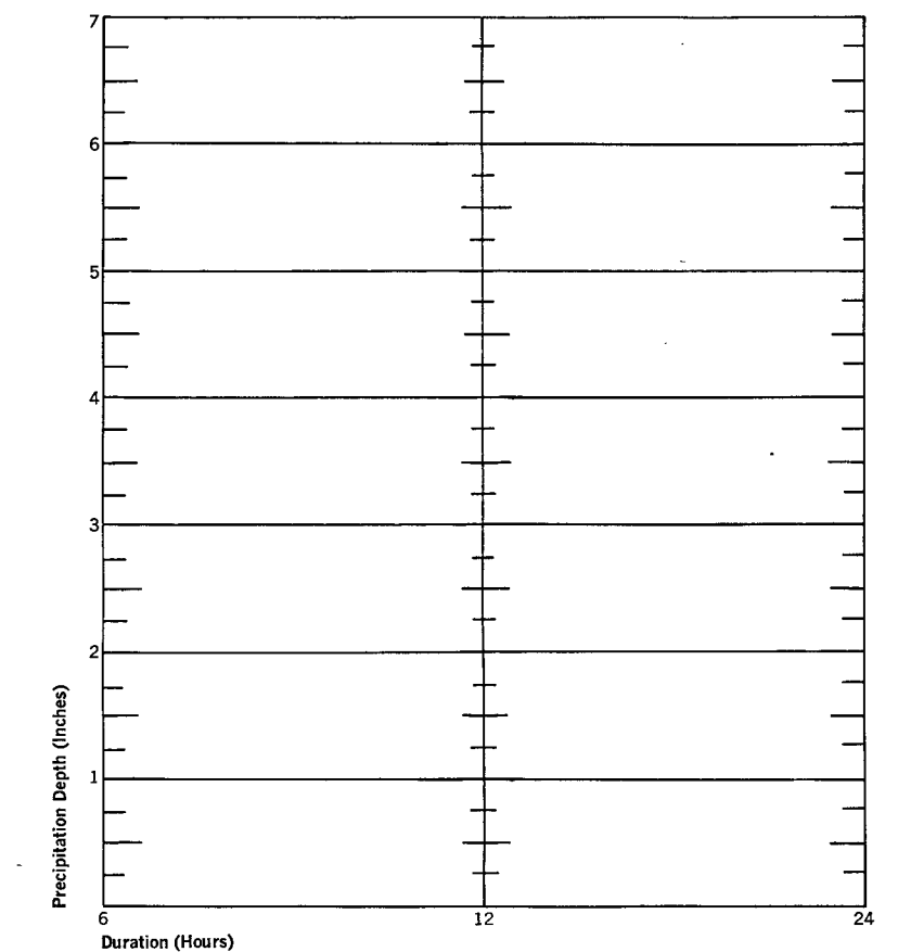
Figure 16. Precipitation depth-duration diagram (6- to 24-hr).
