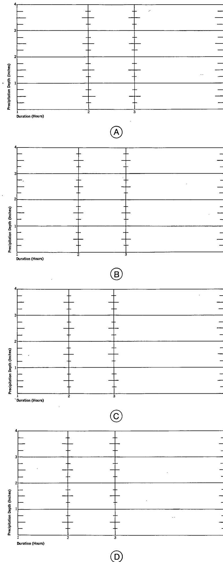
Figure 15. Precipitation depth-duration diagram (1- to 6-hr). a. Virgin River Basin (Region 1, fig. 18). b. Most of Nevada (Region 2, fig. 18). c. Northern Nevada (Region 3, fig. 18). d. Spillover zone from the Sierra Nevada Range (Region 4, fig. 18).
