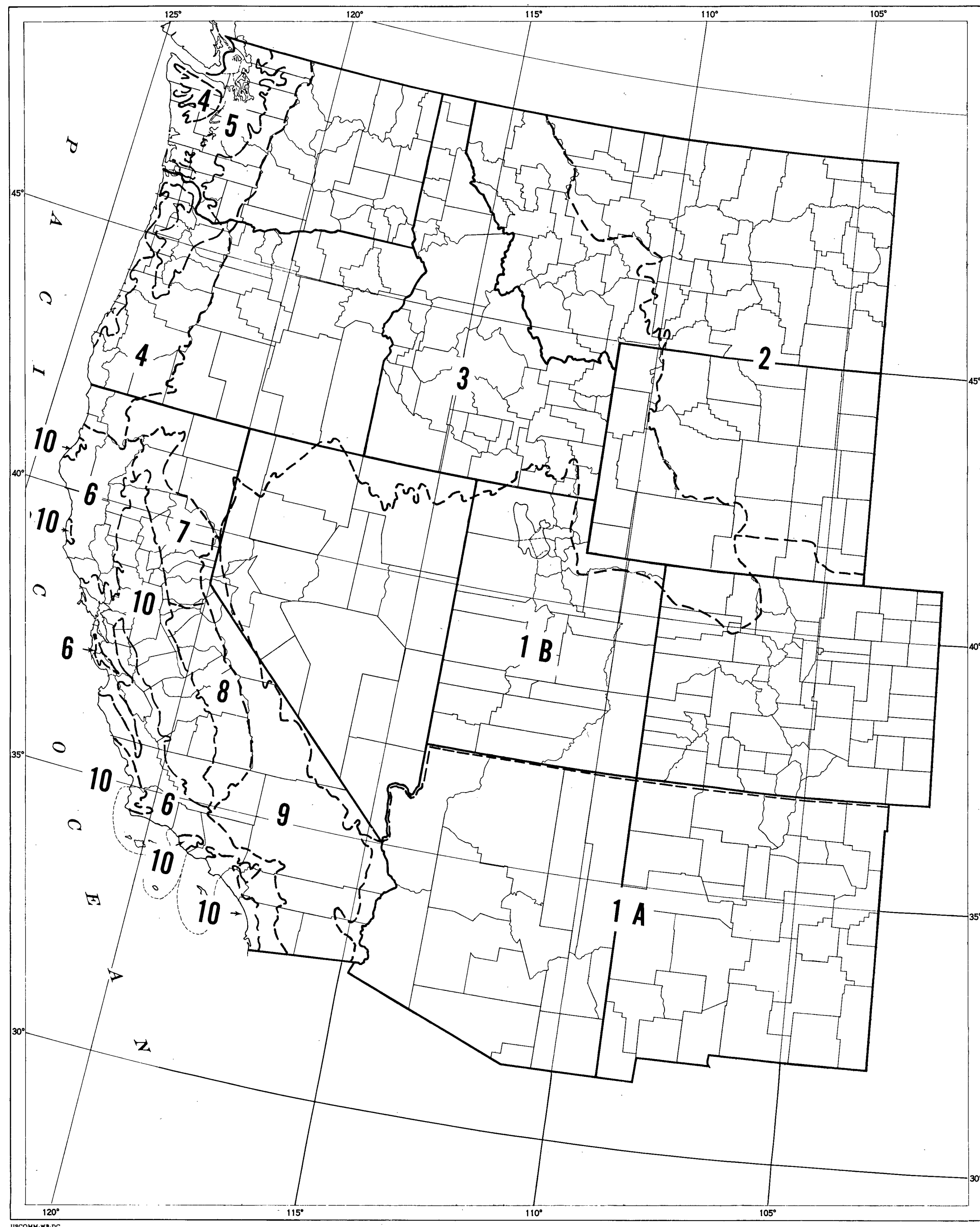
Figure 10. Regions used to develop statistical parameters for interstation interpolation of 2-yr and 100-yr 6-hr precipitation values.
