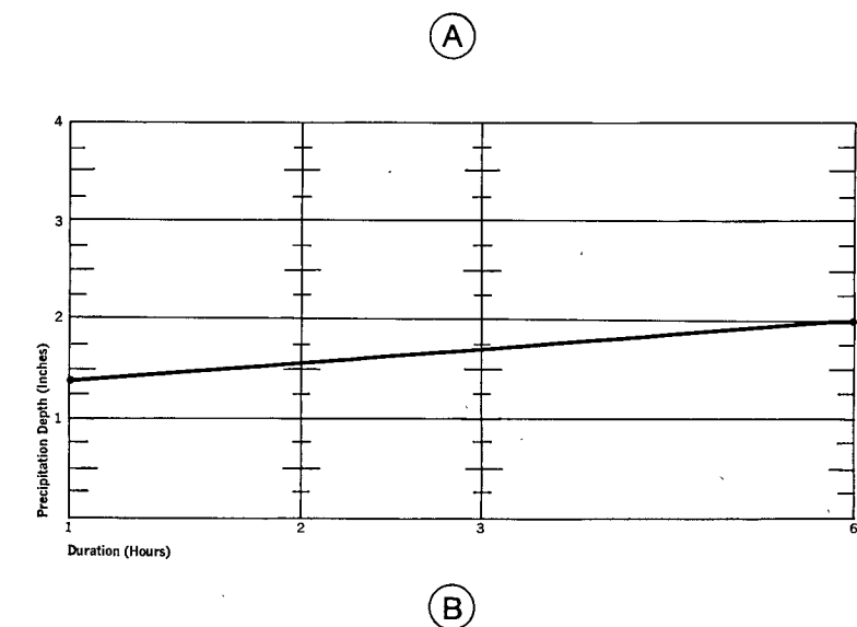
Figure 17. Illustration of use of precipitation-frequency diagrams using values from precipitation-frequency maps and relations.
