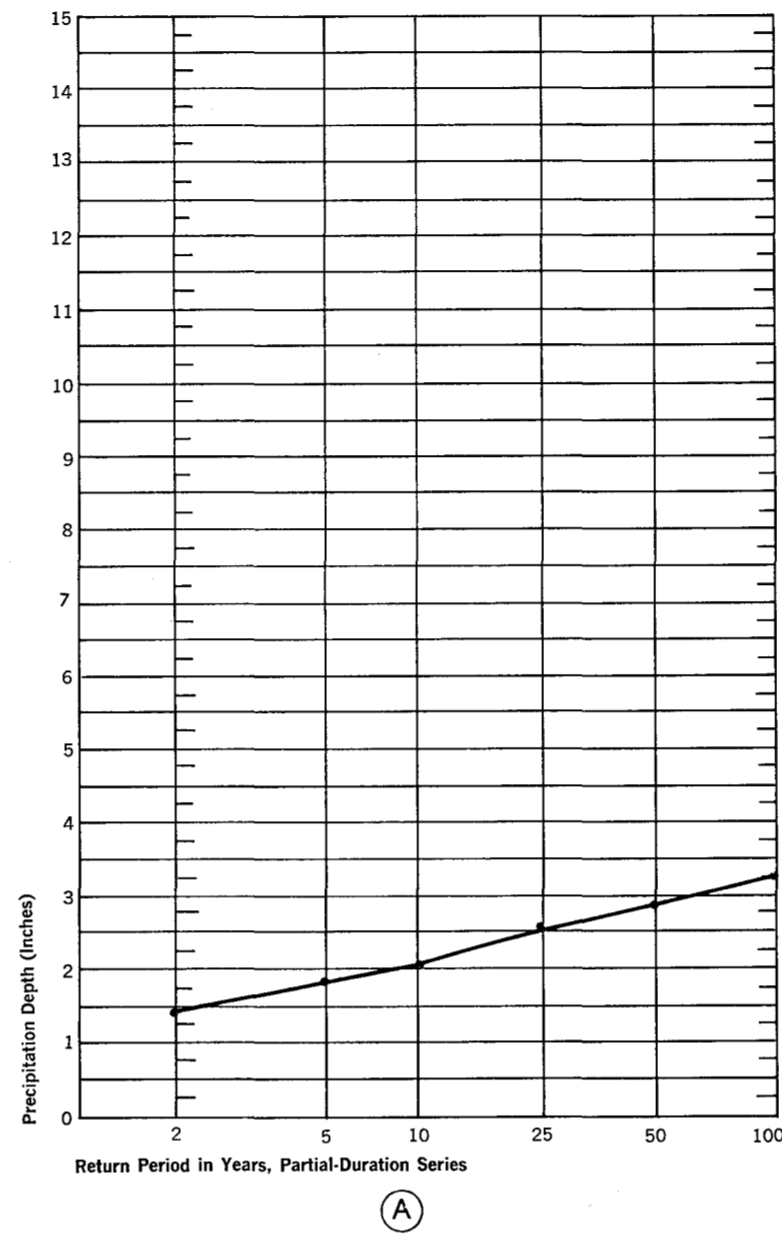
Figure 17. Illustration of use of precipitation-frequency diagrams using values from precipitation-frequency maps and relations at Blanding, Utah.
