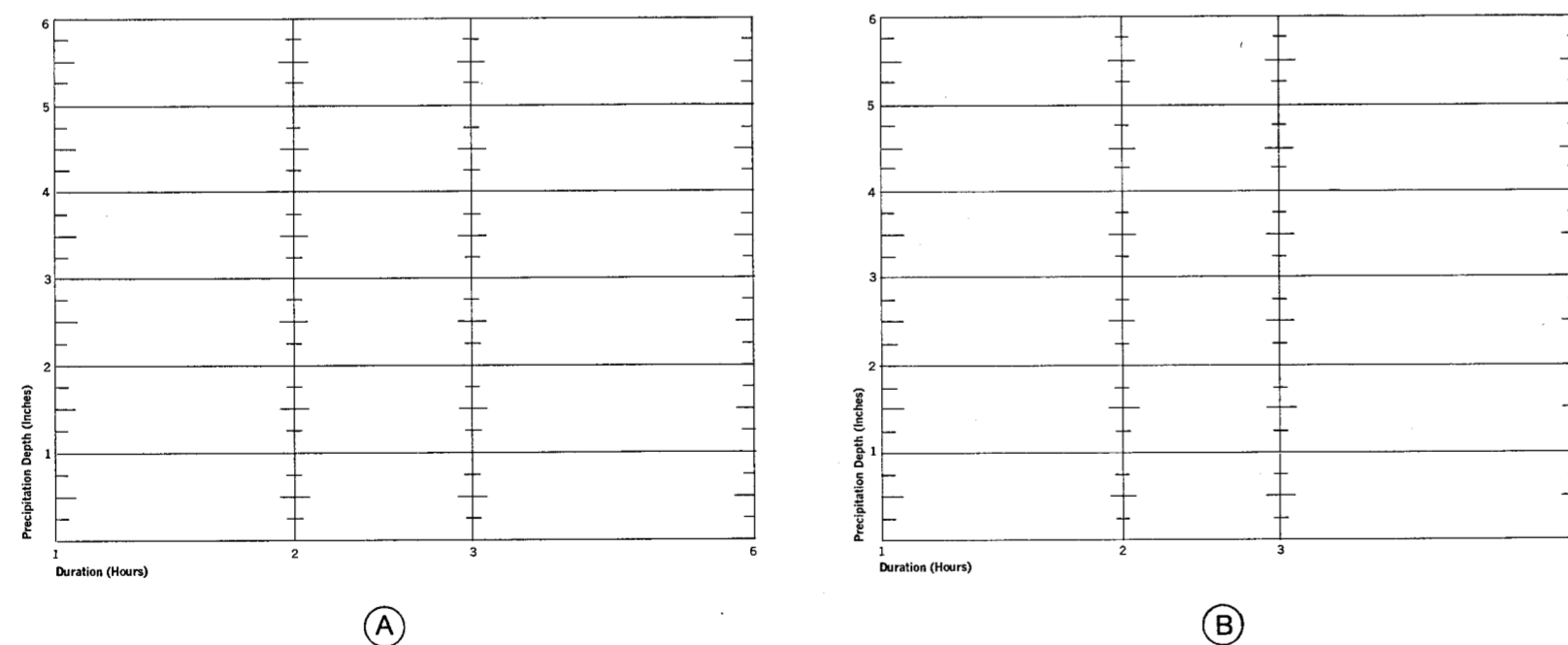
Figure 15. Precipitation depth-duration diagram (1- to 6-hr). a. New Mexico east of generalized crest of Sangre de Cristo Range and Sacramento Mountains (Region 1, fig. 18). b. New Mexico west of generalized crest of Sangre de Cristo Range and Sacramento Mountains (Region 2, fig. 18).
