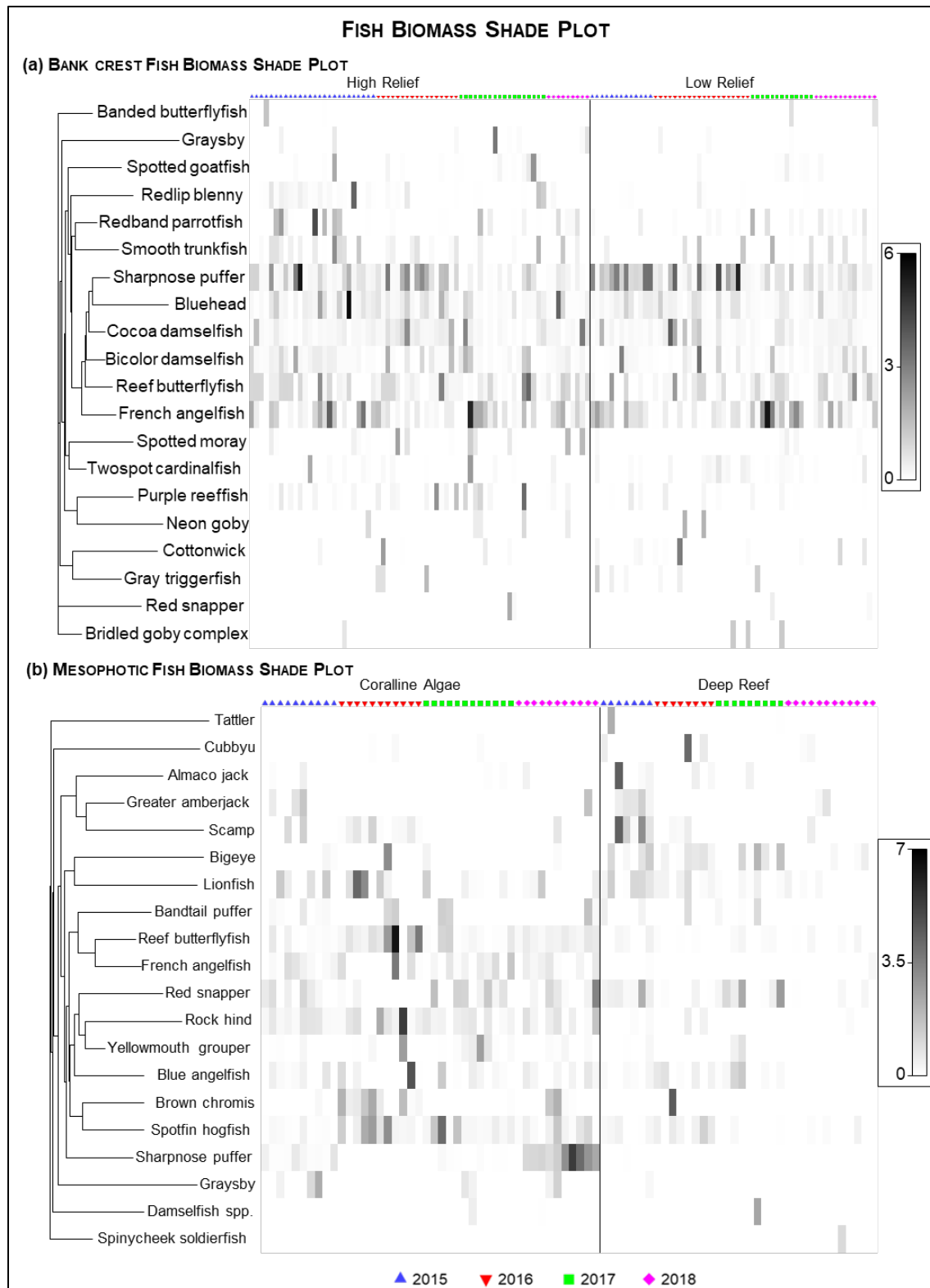
Figure 4.8. Fish species biomass shade plots, where gray scale values represent dispersion weighted biomass, for (a) the bank crest community and (b) the mesophotic community
