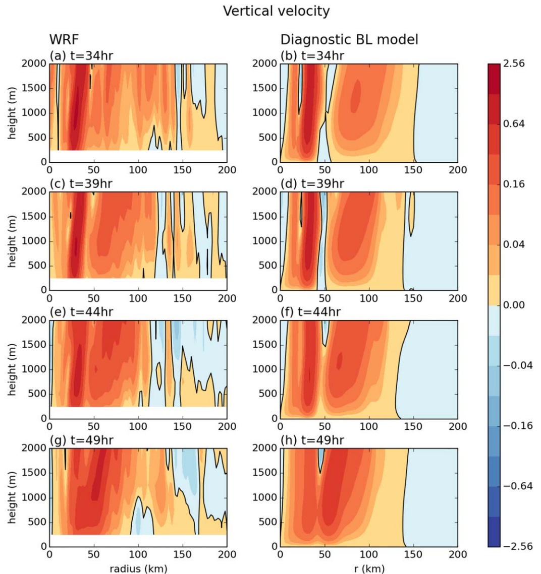
Figure 15. Radius-height sections of vertical velocity. Nonzero contours are in geometric progression, at \pm 0.02, \pm 0.04, \pm 0.08, \dots \pm 2.56 \text{ m s}^{-1} and the zero contour is in black. At 5 h intervals from 34 to 49 h. Left column is WRF ensemble composite FullERC, right is from the KW01 diagnostic model.
