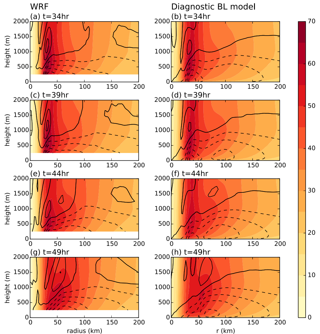
Figure 14. Radius-height sections of azimuthal wind (shading) and radial wind (contours). Contour interval is 5 \text{ m s}^{-1} , negative contours dashed. At 5 h intervals from 34 to 49 h. Left column is WRF ensemble composite FullERC, right is from the KW01 diagnostic model.
