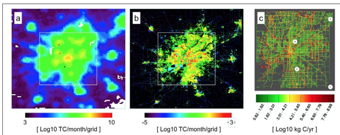
Figure 2: A comparison of three emission fields: 1 × 1 km ODIAC ( a ), 30 × 30 m improved ODIAC emission field (iODIAC) ( b ), and Hestia ( c ). The Figure 2a and 2b indicate the same area as Figure 1. The Hestia emission map (Marion county only) was adopted from Gurney et al. (2012). The numbers on the Hestia map indicate focused emission zones in Gurney et al. (2012). The original high-resolution image is available at the Hestia project web page ( http://hestia.project.asu.edu/index.shtml ). The white box on the ODIAC (a) and iODIAC (b) roughly indicates the Hestia domain in Figure 2c. DOI: https://doi.org/10.1525/elementa.146.f2
