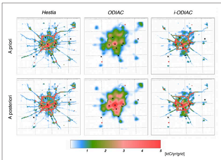
Figure 3: Spatial distributions of a priori (upper) and a posteriori (lower) emissions over Indianapolis, IN. Emission corrections were obtained at a 1 × 1 km resolution. Values are given in the unit of ktC/yr/grid. DOI: https://doi.org/10.1525/elementa.146.f3
