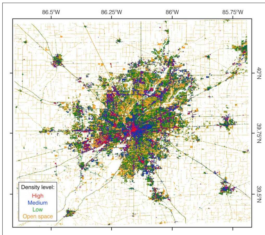
Figure 1: Impervious data over Indianapolis, IN. Data were taken from the National Land Cover Dataset (NLCD, http://www.mrlc.gov/nlcd2011.php ). The impervious data indicate four different levels of developed surface: high intensity (red), medium intensity (blue), low intensity (green) and open-space. According to the NCDC categorization ( http://www.mrlc.gov/nlcd06_leg.php ), high density indicates 80–100% imperviousness, medium indicates 50–79%, low indicates 20–49% and open space indicates less than 20%. DOI: https://doi.org/10.1525/elementa.146.f1
