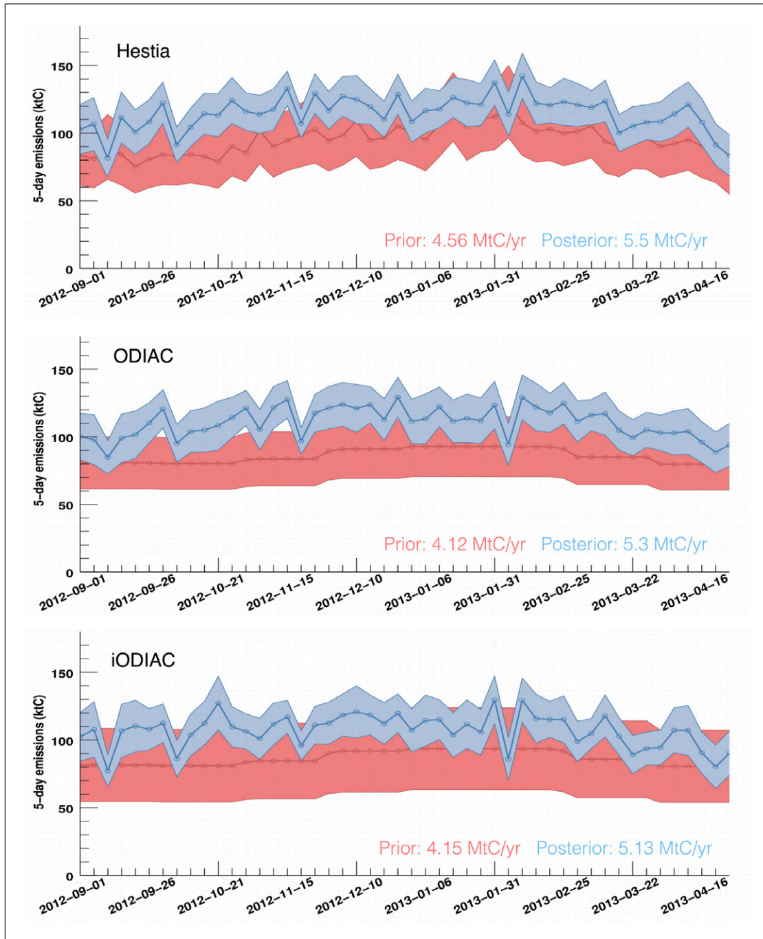
Figure 4: Time series of a priori (in pink) and a posteriori (in blue) emissions of CO 2 aggregated over the Indianapolis inversion domain (indicated in Figure 1) using Hestia (top), ODIAC (middle), and iODIAC (bottom) as prior emissions. DOI: https://doi.org/10.1525/elementa.146.f4
