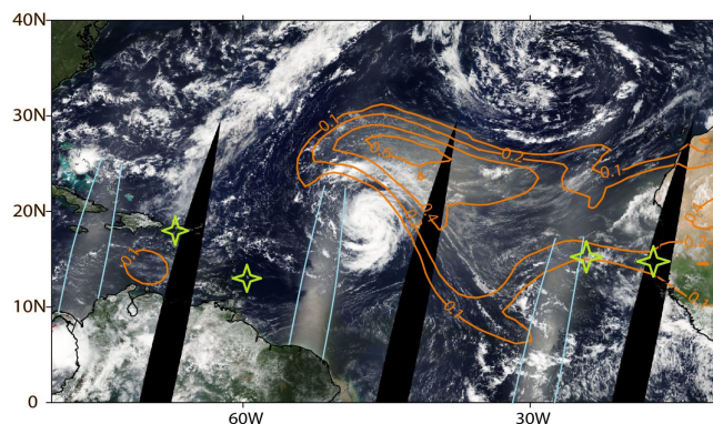
Figure 1. True-color Terra Moderate Resolution Imaging Spectroradiometer (MODIS) satellite imagery composited on 12 September 2012 and overlaid with NAAPS-RA 550 nm dust aerosol optical depth (DAOD, an approximate measure of total atmospheric column of dust aerosol mass, unitless) isopleths, showing Hurricane Nadine's interaction with the SAL. Hurricane Nadine is located in the middle of the image. African dust appears as a light transparent brown haze in between the African coast and Hurricane Nadine, as well as wrapping around the northern periphery of the storm. Note that areas of sunglint (narrow regions between the light blue curves) are similar in color to the dust aerosols but have the same orientation as the satellite orbits and are located approximately midway between satellite coverage gaps (black regions oriented south-southwest to north-northeast). Satellite imagery courtesy of the MODIS flying on NASA's Terra satellite and available from https://worldview.earthdata.nasa.gov/ (last access: 25 November 2020). The stars in light green represent four sites used for validation purposes, including Dakar, Cabo Verde, Ragged Point, and La Parguera in order from east to west.
