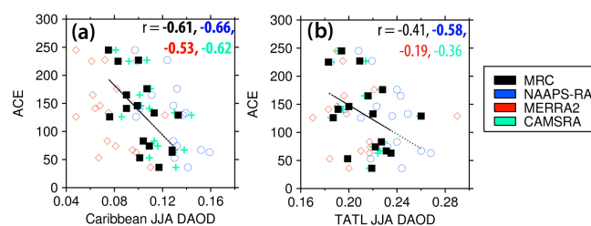
Figure 5. Scatterplot showing the relationship between annual Atlantic accumulated cyclone energy (ACE) and JJA region-averaged DAOD from MRC, NAAPS-RA, MERRA-2, and CAMSRA over the (a) Caribbean and (b) the tropical North Atlantic. One unit of ACE equals 10^4 kt 2 . Correlations ( r ) between ACE and DAOD are color-coded for different DAOD products and overlaid on each plot, and statistically significant correlations are in bold. The possible causes of the DAOD difference between the reanalysis products are discussed in Sect. 3.1.
