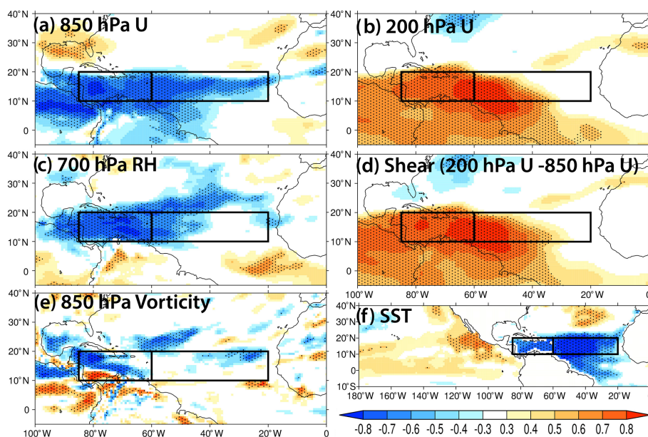
Figure 8. Correlation between MRC JJA regionally averaged DAOD in the Caribbean and JJA (a) 850 hPa U , (b) 200 hPa U , (c) 700 hPa RH, (d) zonal wind shear, (e) 850 hPa relative vorticity, and (f) SST. Correlations over the black dotted areas are statistically significant.
