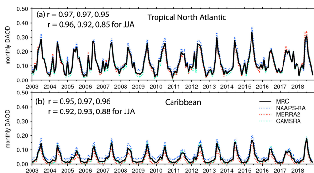
Figure 4. Monthly DAOD at 550 nm from CAMSRA, MERRA-2, NAAPS-RA, and MRC from 2003 to 2018 for the (a) tropical North Atlantic and the (b) Caribbean. Correlations between CAMSRA and MERRA-2, CAMSRA and NAAPS-RA, and MERRA-2 and NAAPS-RA are displayed in sequence for all months and for JJA-only respectively.
