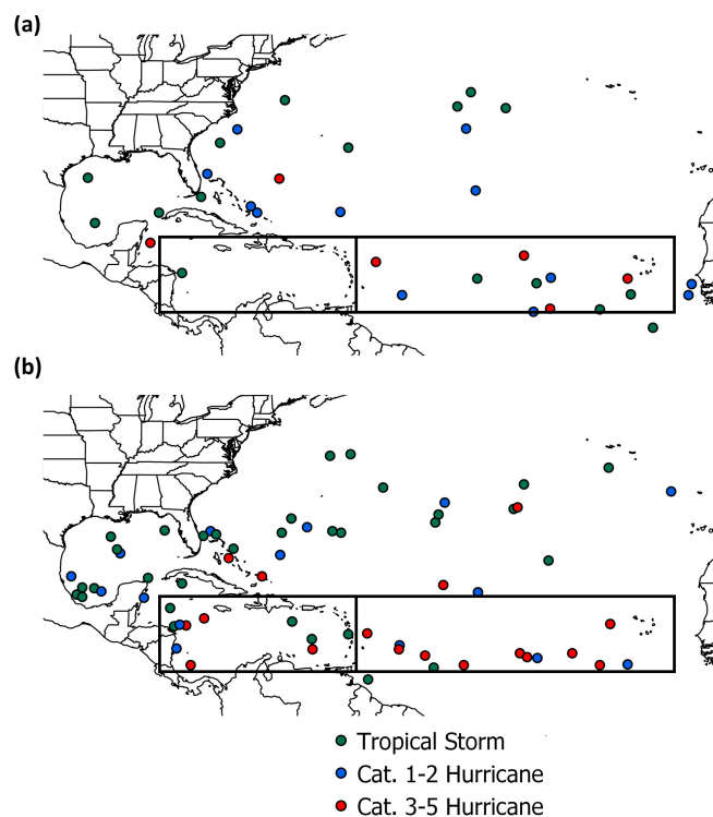
Figure 7. Formation locations of Atlantic named storms during the three seasons with (a) the highest Caribbean JJA DAOD (2014, 2015, and 2018) and (b) the lowest Caribbean JJA DAOD (2005, 2011, and 2017). Also displayed is the maximum intensity that each TC reached.
