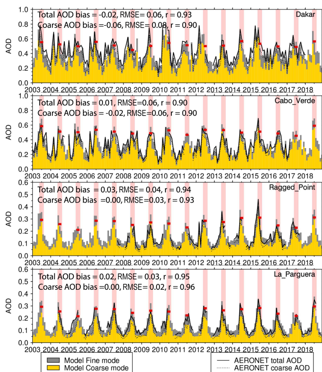
Figure 3. Monthly mean version 3 L2 AERONET and MRC 550 nm modal AODs at four African dust-impacted sites: Dakar, Cabo Verde, Ragged Point, and La Parguera from east to west. JJA are highlighted with pink shading, and JJA seasonal average total AODs from MRC are shown with red bars. Annotations for each time series show bias, RMSE, and correlation ( r ) of monthly averages calculated from the MRC.
