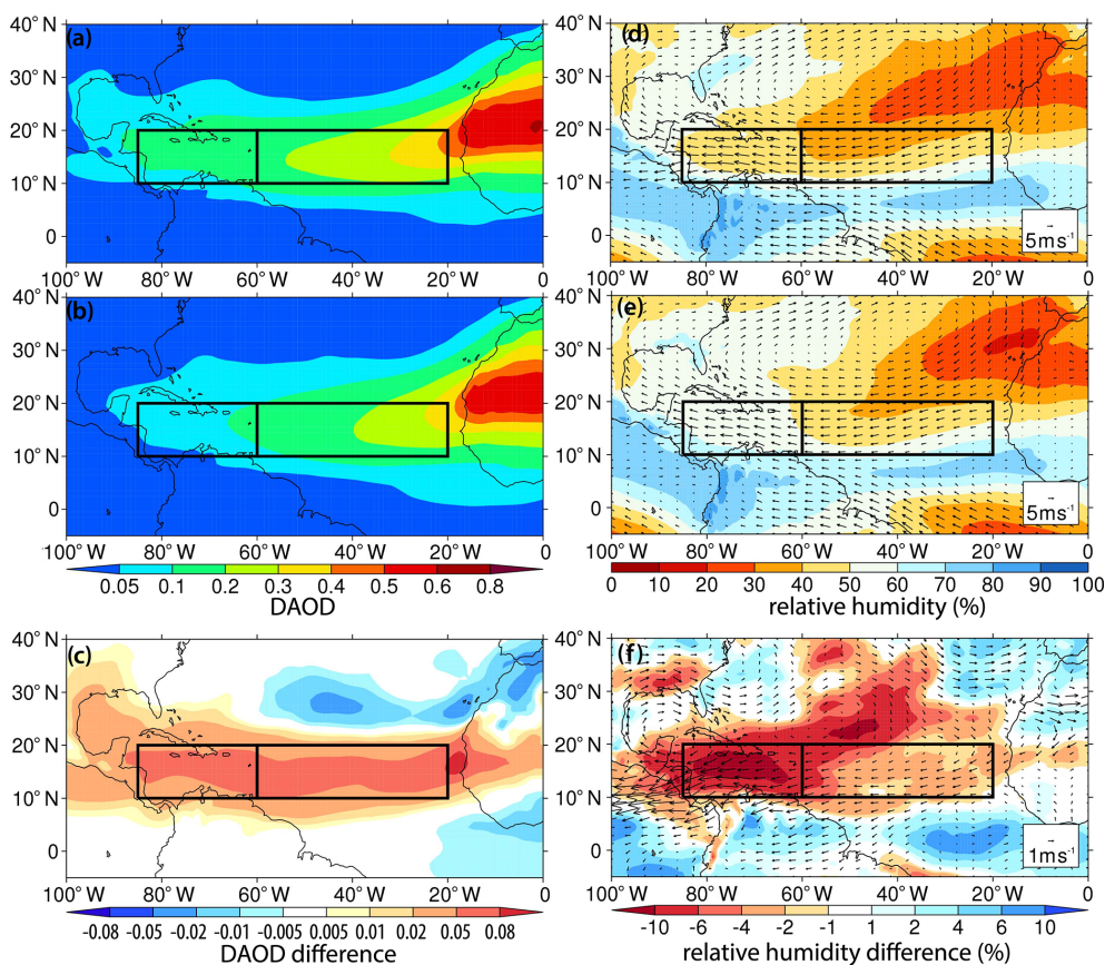
Figure 6. (a, b, c) MRC JJA composite of DAOD for the three Atlantic hurricane seasons from 2003 to 2018 with (a) the highest JJA Caribbean DAOD (2014, 2015, and 2018), (b) the lowest JJA Caribbean DAOD (2005, 2011, and 2017), and (c) the difference between the two (highest minus lowest). (d, e, f) the corresponding JJA composite of 850 hPa wind (vectors) and 700 hPa RH (color shading).
