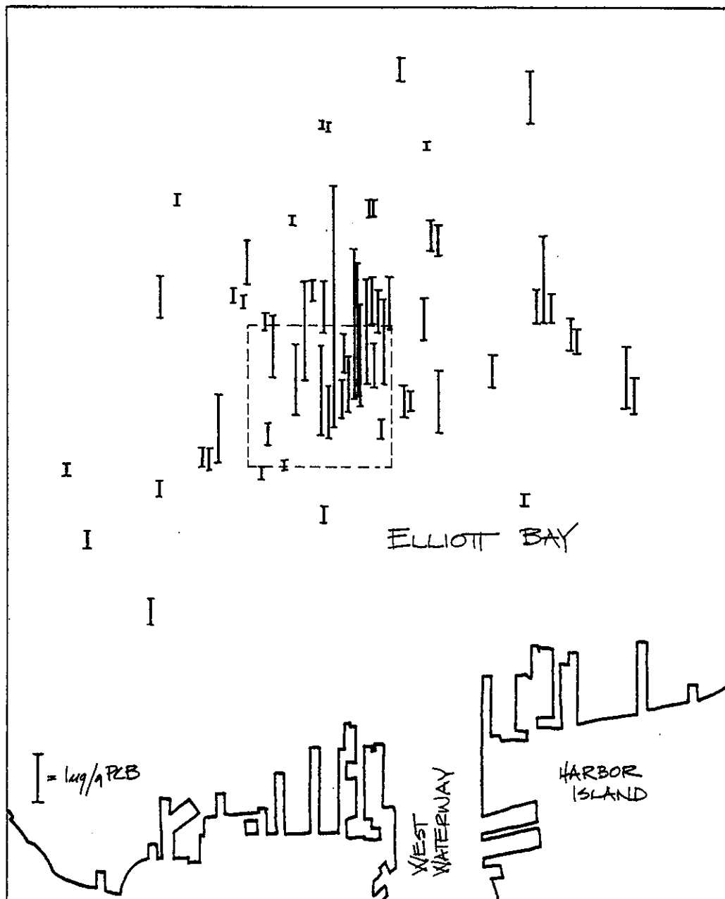
Figure IX-6. Concentrations of PCBs Observed in the Sediments of Southern Elliott Bay. Dashed Square Indicates the Location of a PCB-Contaminated Dredged-Material Mound.
