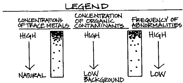
Figure d. Approximate Distributions in Puget Sound of Trace Metals, Organic Contaminants and Increased Incidences of Abnormalities in Benthic Organisms.
