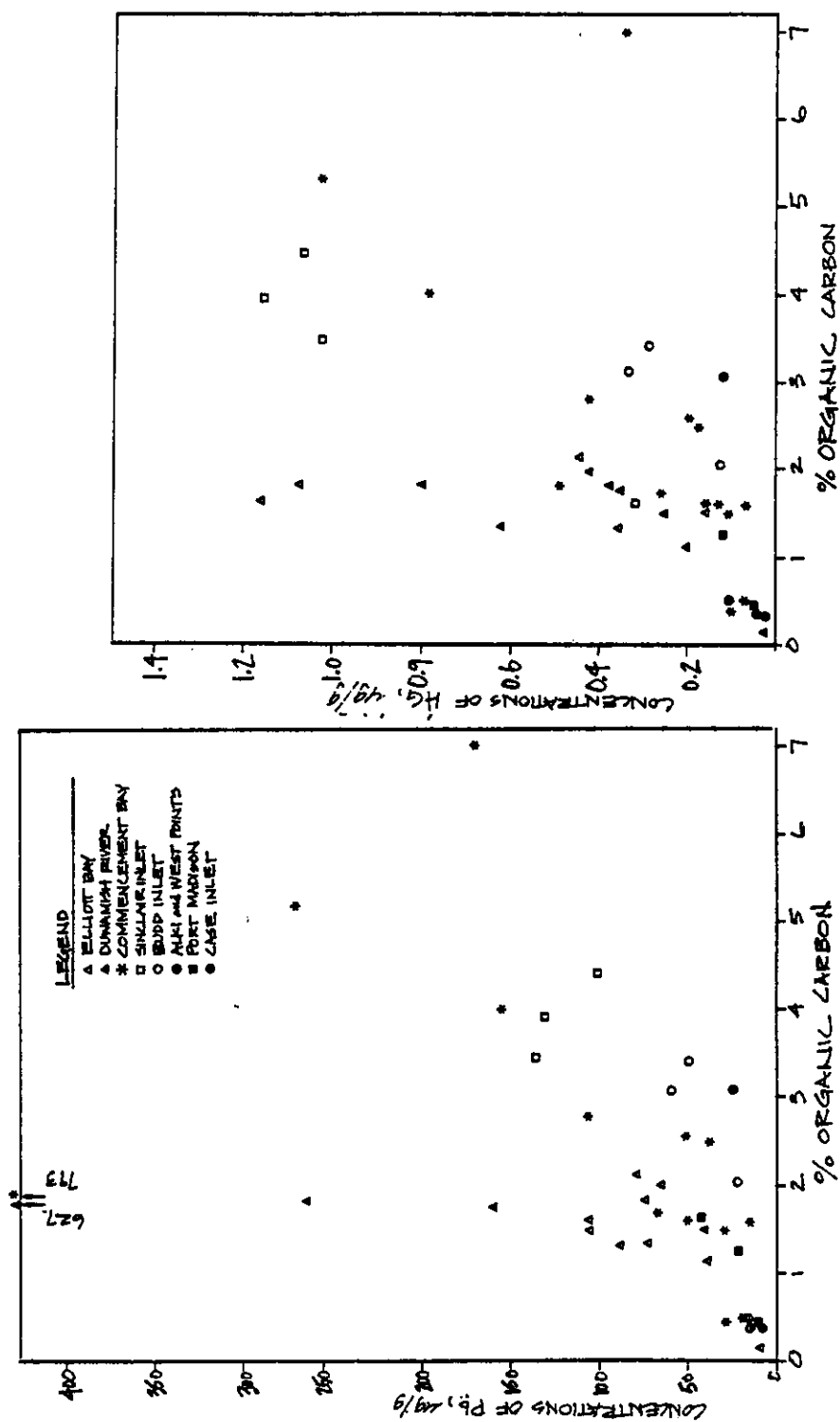
Figure VIII-10. Scattergrams of the Concentrations of Pb and Hg Observed in the Sediments versus the Percent Organic Matter.
