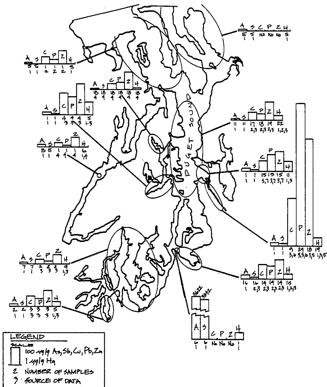
Figure VIII-1. Averaged Concentrations of Selected Trace Metals Observed in the Sediments of Puget Sound.
