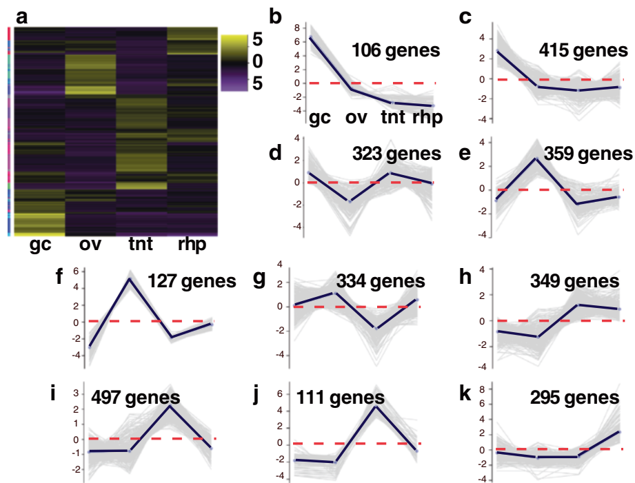
Fig. 3 a-k Heatmap of A. alata medusa samples. Hierarchical clustering (EdgeR) and corresponding ten subcluster profiles for the 2916 genes differentially expressed across A. alata medusa samples (gastric cirri, ovaries, tentacle (with pedalius base), rhopalium) (of the identified ~20 K Trinity genes). Intensity of color indicates expression levels for each of the ten hierarchical clusters (vertical access). Bright yellow patches correspond to the highest peaks for each k-mean subcluster profile. K-mean profiles ( b-k ) match the order of column names in a , representing the mean expression of gene clusters highly abundant in each sample (centroid demarcated by the solid line; zero indicated by the horizontal dashed red line). Three bright yellow transcript clusters in the gastric cirri column correspond to each of the peaks seen in plots b , c and d in the ovaries column correspond to plots e , f , g and in the tentacle column correspond to h , i , j , while the two bright yellow clusters in the rhopalium column correspond to peaks in plots k , and to the less prominent peaks in plots g and h . The vertical colored bar on the left of the heatmap ( a ) indicates distinct patterns corresponding to the ten subcluster profiles (sc = subcluster number), for which the number of genes each comprises is indicated. Abbreviations: gc = gastric cirri, ov = ovaries, tnt = tentacle (and pedalius base), rhp = rhopalium, and pln = planulae. (Original matrix in Additional file 5)
