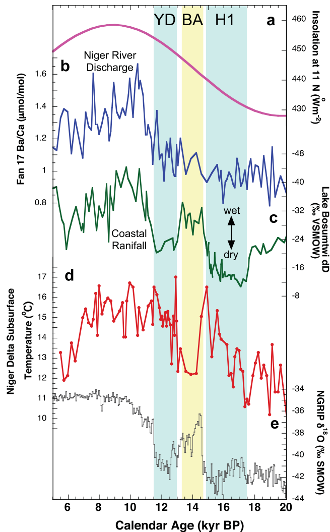
Figure 6. West African Monsoon variability across the deglaciation. (a) Northern Hemisphere summertime insolation at 11°N, (b) Fan 17 G. ruber Ba/Ca ( \mu\text{mol/mol} ) record reflecting changes in Niger River discharge across the deglaciation 14 (c) Lake Bosumtwi \delta D_{\text{leaf wax}} (‰ VSMOW) (ref. 36 ) (d) , Fan 17 subsurface temperature record and (e) NGRIP ice core record 51 . Note that precipitation changes recorded in the Lake Bosumtwi \delta D_{\text{leaf wax}} record correspond to subsurface warming in the Niger Delta, most likely resulting from increased SSTs in the EEA cold tongue and reduced precipitation over land.
