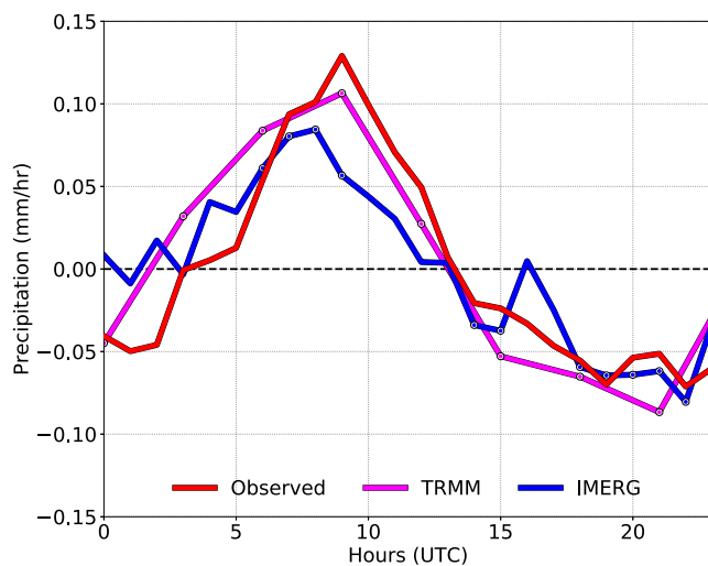
Figure 14. Hourly composites of IMERG area-averaged precipitation rates (blue), TRMM area-averaged precipitation rates (magenta), and PIRATA observations (red) at 8°N, 38°W for JJA. Circles show when hourly IMERG and TRMM values are significant with 95% confidence based on a two-tailed t test.
