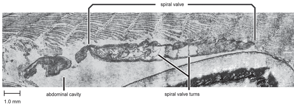
FIGURE 6. Mollisquama mississippiensis sp. nov. spiral valve detail (a single synchrotron scan layer); anterior is to the right.
