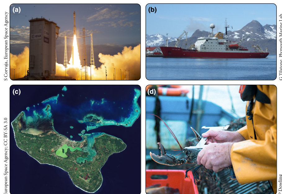
Figure 1. (a) An environmental monitoring satellite is launched into a polar orbit. (b) Research vessels, buoys, and transport ships all routinely collect measurements for monitoring ocean atmosphere–ocean gas exchange, but some oceans are not well sampled and much of the data collection is voluntary. (c) A coral reef viewed from space; these sensitive ecosystems can be negatively impacted by episodic ocean acidification events caused by upwelling (Feely et al. 2008). (d) Calcifying organisms that use carbonate to build their shells, including commercially important lobsters, can be negatively affected by ocean acidification (McLean et al. 2018).
