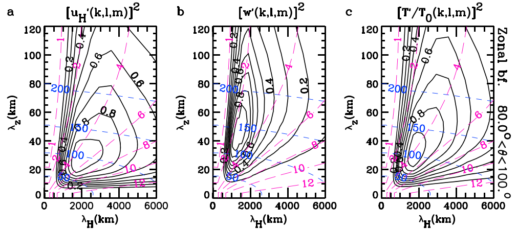
Figure 3. Power spectral density amplitudes, equation (37), of the compressible solutions shown in Figure 2a for the secondary gravity waves having azimuths of 80\text{--}100^\circ . (a) Horizontal velocity spectrum: |\widetilde{u}'_H|^2 \Delta k \Delta l \Delta m . (b) Vertical velocity spectrum: |\widetilde{w}'|^2 \Delta k \Delta l \Delta m . (c) Temperature perturbation spectrum: |\widetilde{T}'/\widetilde{T}|^2 \Delta k \Delta l \Delta m . Each spectrum is normalized by its maximum value (which is arbitrary) and is shown in 10% increments of its maximum value as solid lines. Blue short dashed lines show c_{iH} in 50 m/s increments, and pink long dashed lines show \tau_{ir} in hours.
