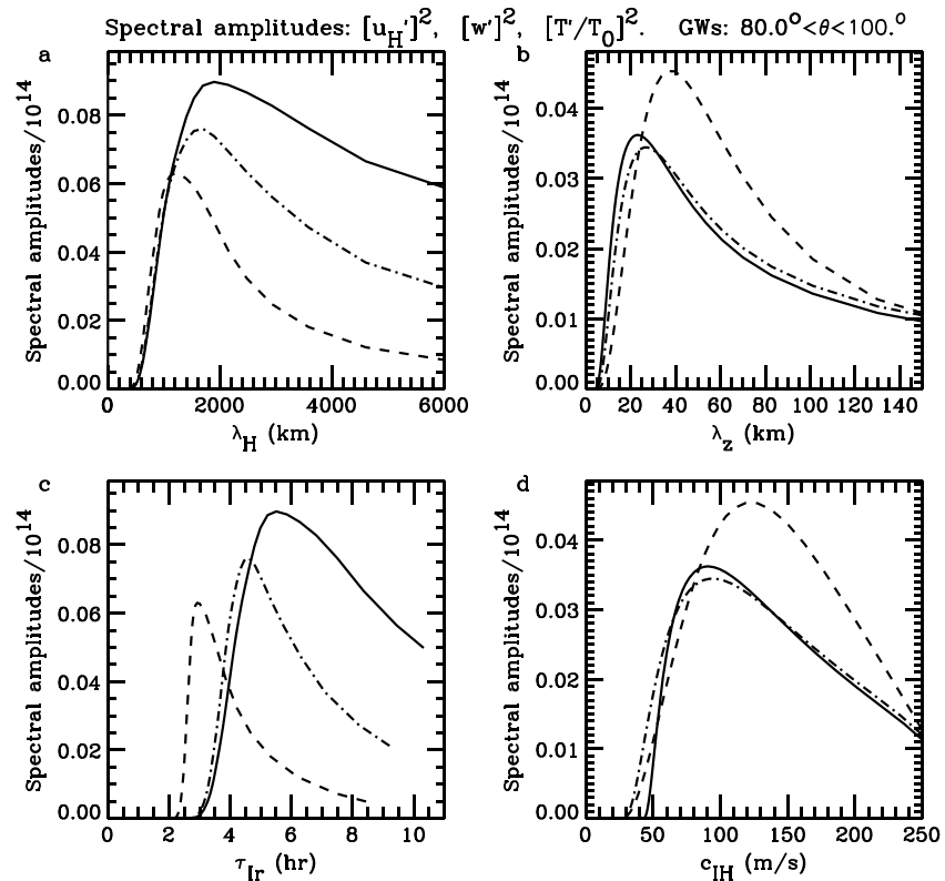
Figure 4. The 1-D spectra for the compressible solutions shown in Figure 3 for the secondary gravity waves (GWs) having azimuths of 80–100°. Solid, dashed, and dash-dotted lines show \Sigma|u'_H|^2 \Delta k \Delta / \Delta m , \Sigma 3,000|w'|^2 \Delta k \Delta / \Delta m , and \Sigma 3 \times 10^5 |\tilde{T}' / \bar{T}|^2 \Delta k \Delta / \Delta m , respectively. These amplitudes are shown as functions of (a) \lambda_H , (b) |\lambda_z| , (c) \tau_{lr} , and (d) c_{lH} .
