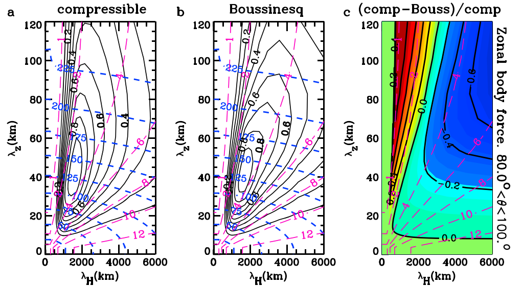
Figure 2. Compressible (a) and Boussinesq (b) vertical flux of horizontal momentum for the secondary gravity waves having azimuths of 80\text{--}100^\circ excited by a zonal body force centered at z_0 = 45 m with D_H = 800 km, D_z = 8 km, and \chi = 2 hr. Each spectrum is normalized by its maximum value (which is arbitrary) and is shown in 10% increments of its maximum value (solid black lines). Blue short dashed lines indicate the intrinsic horizontal phase speed, c_{lH} , in 25 m/s intervals. (c) (Compressible-Boussinesq)/compressible fluxes from (a) and (b) (solid black lines). Pink long dashed lines show gravity wave intrinsic periods, \tau_{lr} , in hours.
