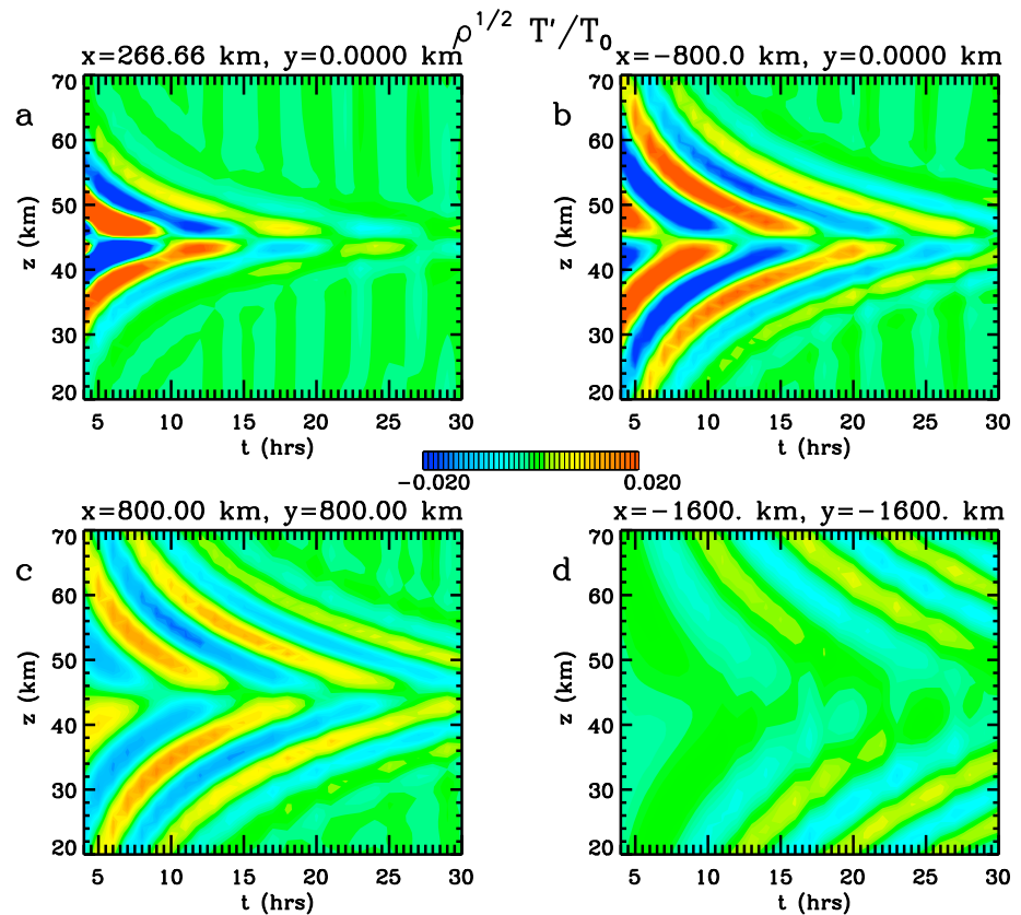
Figure 13. The scaled temperature perturbations, \sqrt{\bar{\rho}} T' / \bar{T} (in \sqrt{g/m^3} ), for the same zonal body force with \chi = 2 hr as in Figure 7 at (a) x = 267 km and y = 0 , (b) x = -800 km, and y = 0 , (c) x = 800 km and y = 800 km, and (d) x = -1,600 km and y = -1,600 km.
