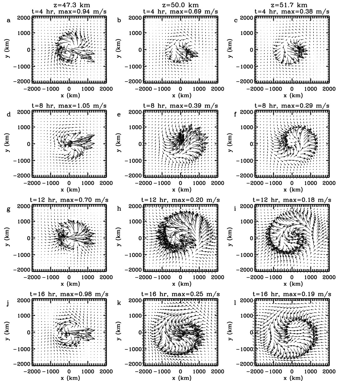
Figure 10. The total (gravity wave plus mean responses) horizontal velocity induced by the same zonal body force as in Figure 7. (a–c) The horizontal velocity at t = 4 hr at z = 47.3, 50.0, and 51.7 km, respectively. The arrows show the direction, and the lengths are proportional to the magnitude. (d–f, g–i, and j–l) show the same as the first row but for t = 8, 12, and 16 hr, respectively. The maximum amplitude in each panel is labeled.
