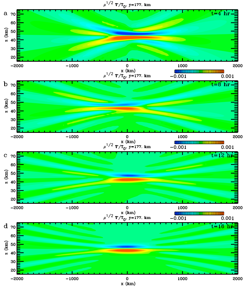
Figure 7. \sqrt{\bar{\rho}} T' / \bar{T} (in \sqrt{g/m^3} ) for the secondary gravity waves plus mean temperature perturbations created by the zonal body force with \chi = 2 hr at y = 177 km. (a) t = 4 hr. (b) t = 8 hr. (c) t = 12 hr. (d) t = 16 hr.
