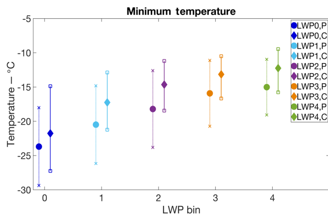
Figure 5. Mean minimum cloud temperature for clean and polluted clouds for each LWP bin. Diamond markers with solid line indicate clean clouds; circle markers with dashed line represent polluted cases. The bars span the 20–80th percentile of the T_{\min} distribution for each bin.
