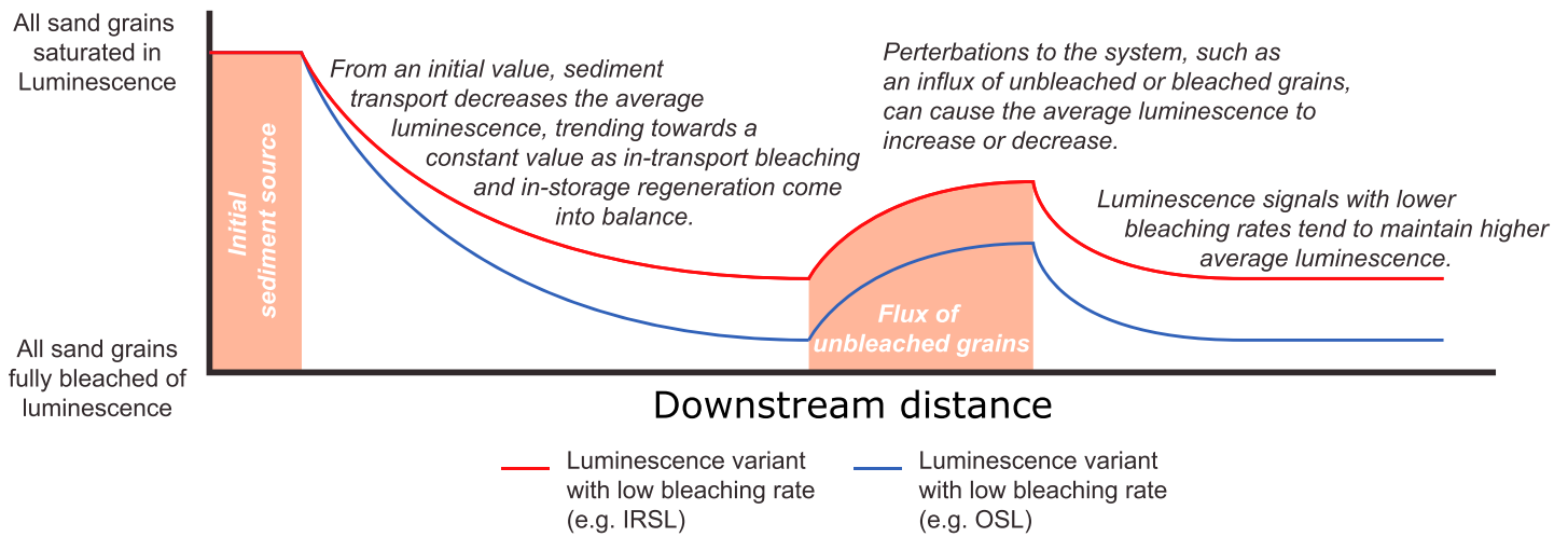
Figure 7. Schematic patterns of the luminescence averaged over thousands of grains in an idealized channel/floodplain fluvial system. Adapted from Gray et al. (2017).
