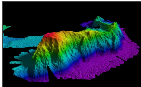
Figure 1. Bathymetric survey of an Arctic seamount
