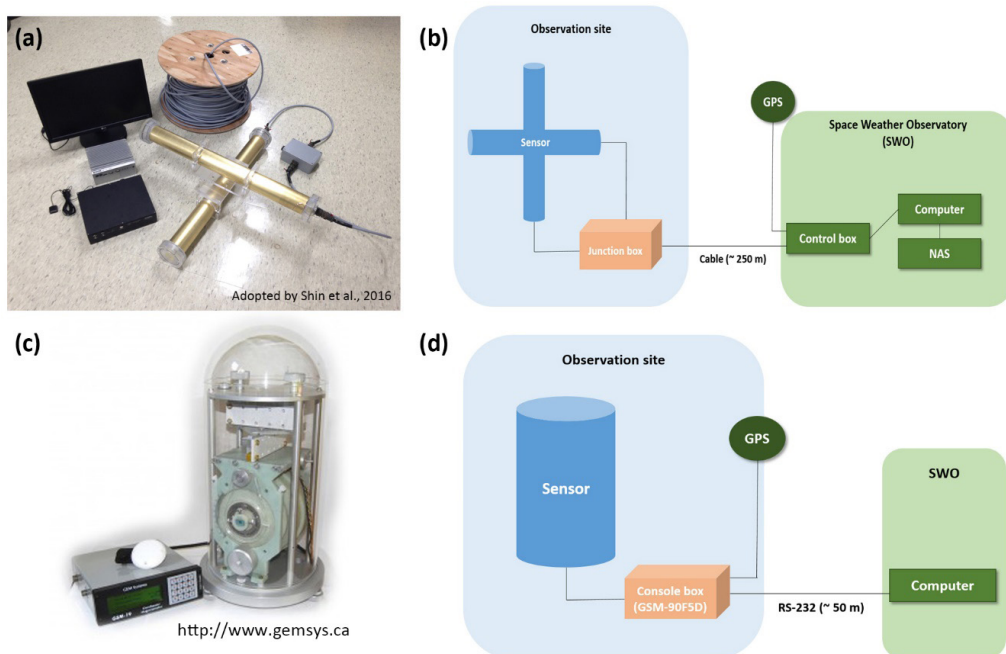
Fig. 5. (a) Components of the search-coil magnetometer (SCM) and (b) block diagrams for the SCM. (c) Components and (d) block diagrams for the vector magnetometer, dIdD.
