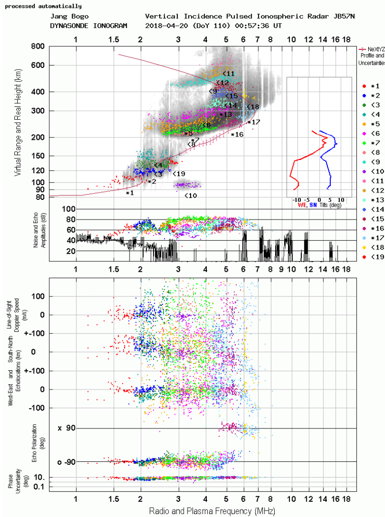
Fig. 4. A VIPIR ionogram from 00:57 UT on April 20, 2018. The explanations for each plot are written in text.
