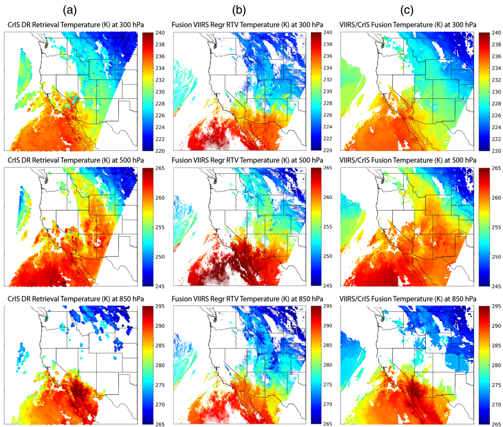
Fig. 1 Temperature (K) is shown at 300, 500 and 850 hPa in the top, middle and bottom panels, respectively. (a) CrIS DR retrievals at sounder resolution, (b) regression retrievals derived from VIIRS/CrIS fusion radiances at imager resolution, and (c) VIIRS/CrIS fusion products at imager resolution. On April 10, 2018, at 0936 and 0942 UTC (CrIS granule start times).
