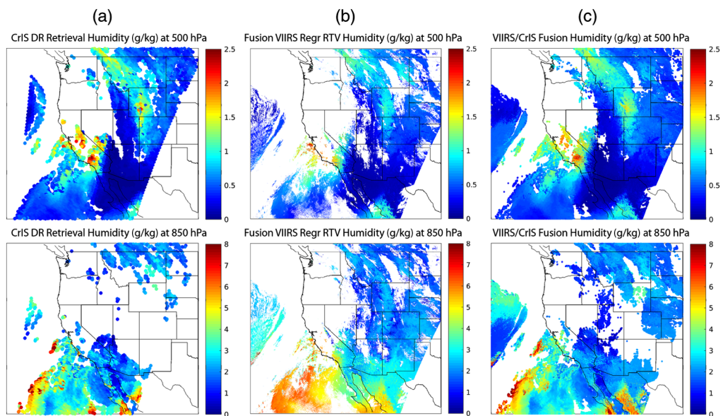
Fig. 2 H 2 O mixing ratio (g/kg) is shown at 500 and 850 hPa in the top and bottom panels, respectively. (a) CrIS DR retrievals at sounder resolution, (b) regression retrievals derived from VIIRS/CrIS fusion radiances at imager resolution, and (c) VIIRS/CrIS fusion products at imager resolution. On April 10, 2018, at 0936 and 0942 UTC (CrIS granule start times).
