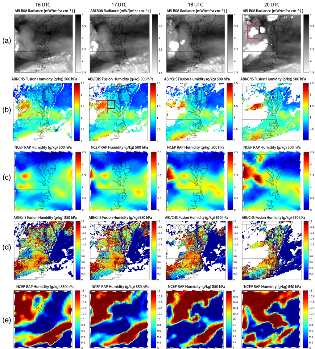
Fig. 7 ABI band 8 ( 6.3 \mu\text{m} ) radiance ( \text{mW m}^{-2} \text{sr}^{-1} \text{cm} ) is shown in (a), ABI/CrIS 8-band product fusion \text{H}_2\text{O} (g/kg) at 500 hPa and 850 hPa is shown in (b) and (d), respectively, whereas the 13-km RAP analysis \text{H}_2\text{O} product at 500 and 850 hPa is shown in (c) and (e), respectively. The high (low) moisture feature at 17 UTC inside the red (black) box in (b) and (d) corresponds to the existing cloud development in the red box (new convection in the black box) outlined at 20 UTC in (a).
