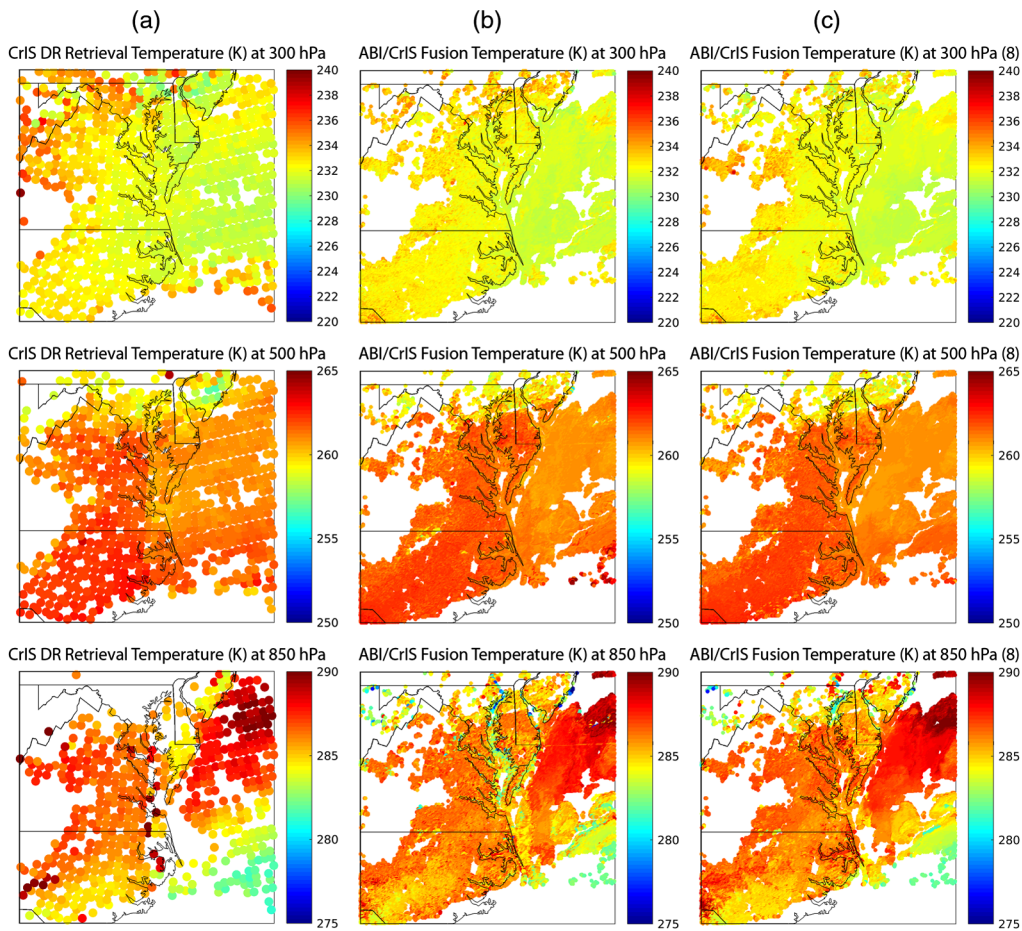
Fig. 5 Temperature (K) is shown at 300, 500, and 850 hPa in the top, middle, and bottom panels, respectively; (a) CrIS DR retrievals at sounder resolution, (b) ABI/CrIS fusion results using a two-band (split-window) k-d tree search, and (c) ABI/CrIS fusion results using an eight-band k-d tree search. On May 19, 2017, ABI data are from 1800 UTC and CrIS data are from 1748 and 1754 UTC.
