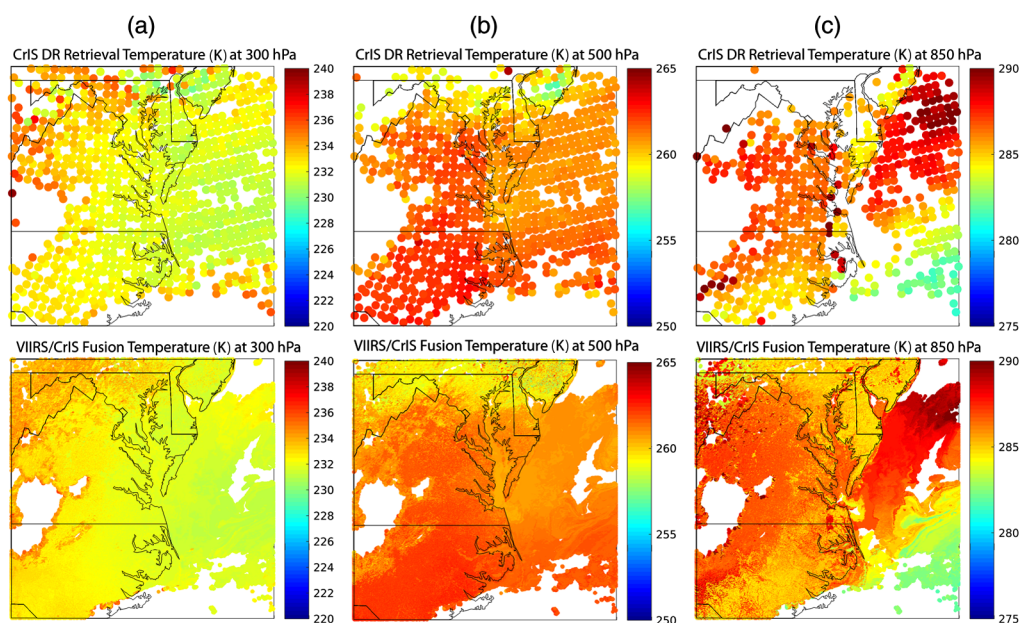
Fig. 3 Temperature (K) provided by the CrIS DR retrieval (top) and the VIIRS/CrIS product fusion (bottom) is shown at the 300, 500, and the 850 hPa pressure level in panels (a), (b), and (c), respectively. On May 19, 2017, at 1748 and 1752 UTC (CrIS granule start times).
