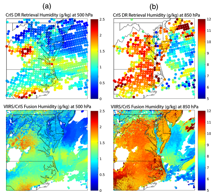
Fig. 4 H 2 O mixing ratio (g/kg) provided by the CrIS DR retrieval (top) and the VIIRS/CrIS product fusion (bottom) at the 500 and 850 hPa pressure level in panels (a) and (b), respectively. On May 19, 2017, at 1748 and 1752 UTC (CrIS granule start times).
