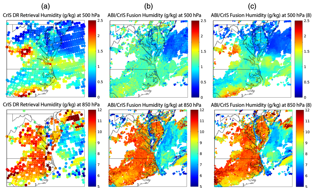
Fig. 6 H 2 O mixing ratio (g/kg) is shown at 500 and 850 hPa in the top and bottom panels, respectively; (a) CrIS DR retrievals at sounder resolution, (b) ABI/CrIS fusion results using a two-band (split-window) k-d tree search, and (c) ABI/CrIS fusion results using an eight-band k-d tree search. On May 19, 2017, ABI data are from 1800 UTC and CrIS data are from 1748 and 1754 UTC.
