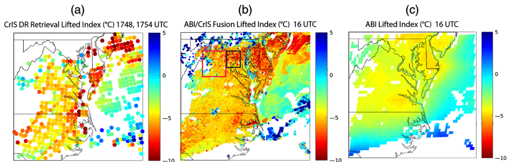
Fig. 8 (a) CrIS DR LI ( ^{\circ}\text{C} ) retrievals derived at CrIS measurement times 1748 and 1754 UTC on May 19, 2017. (b) ABI/CrIS fusion LI ( ^{\circ}\text{C} ) from 2 h earlier (using the ABI images at 16 UTC) (with the red and black boxes delineating more stable and less stable atmospheres associated with those in Fig. 7). (c) ABI only LI ( ^{\circ}\text{C} ) at 16 UTC.
