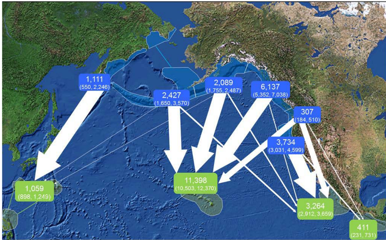
Figure 4. Abundance by summer feeding areas (blue), and winter breeding areas (green), with 95% confidence limits in parentheses. Migratory destinations from feeding area to breeding area are indicated by arrows with width of arrow proportional to the percentage of whales moving into winter breeding area (Wade et al. 2016).
