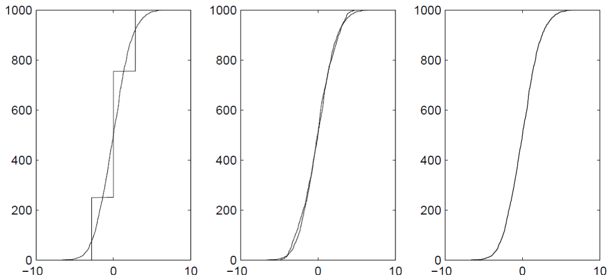
Figure 4. Comparison of results of computing a random walk after 2 steps.
