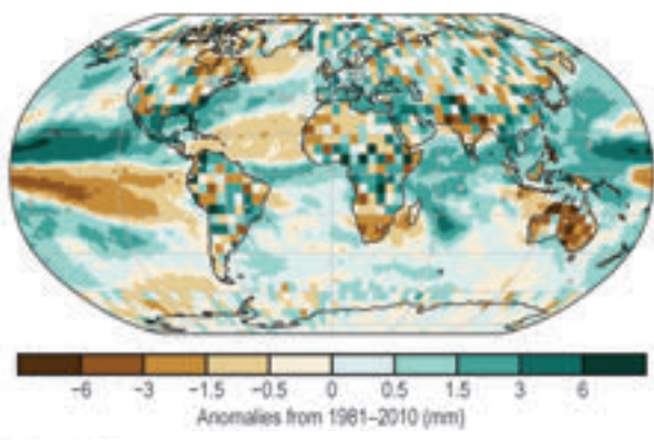
(k) Precipitation
