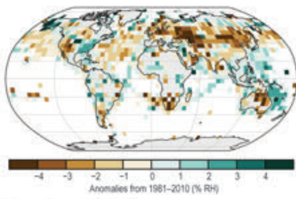
(j) Upper Tropospheric Humidity
