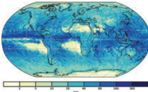
FIG. 2.22. Maximum 1-day precipitation amount (Rx1day, mm) for 2018 from ERA5.
