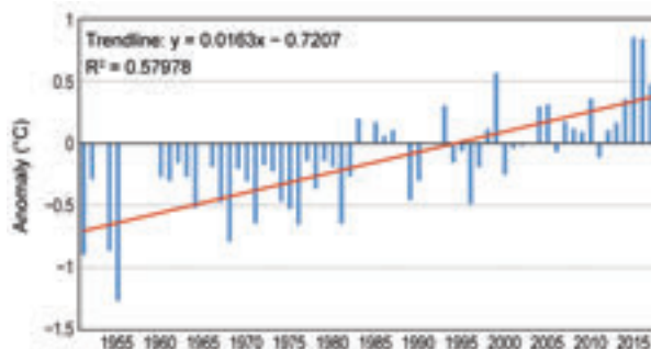
FIG. 7.26. Annual mean temperature anomalies ( ^{\circ}\text{C} ; base period: 1981–2010) of 26 climate stations in South Africa, for the period 1951–2018. Red line represents the linear trend. (Source: South African Weather Service.)
