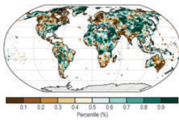
(n) Cloudiness
