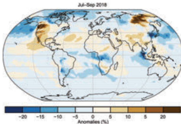
FIG. 2.62. Jul–Sep total column CO anomaly (%) for 2018 with respect to the Jul–Sep 2003–18 median from the CAMS interim reanalysis.
