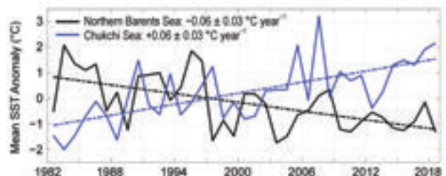
FIG. 5.7. Area-averaged SST anomalies ( ^{\circ}\text{C} ) for Aug of each year relative to the 1982–2010 Aug mean for the Chukchi Sea region ( 68^{\circ} – 74^{\circ}\text{N} , 180^{\circ} – 200^{\circ}\text{E} ) and the northern Barents Sea region ( 76.4^{\circ} – 79.4^{\circ}\text{N} , 38^{\circ} – 60^{\circ}\text{E} ); regions are shown by black dashed lines in Fig. 5.5a. Dashed lines show linear SST anomaly trends over the period shown. Numbers in the legend correspond to linear trends in ^{\circ}\text{C yr}^{-1} (with 95% confidence intervals).
