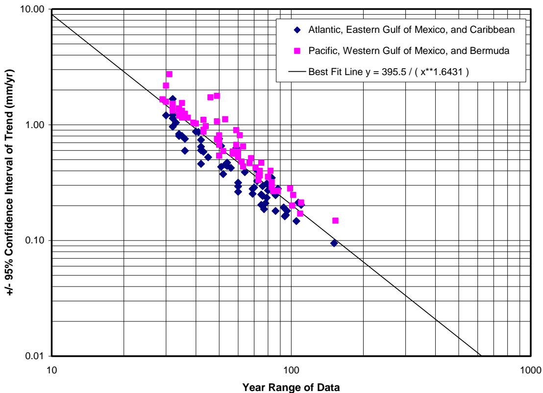
Figure 29. +/- 95% confidence interval of linear MSL trends (mm/yr) versus year range of data. The least squares fitted line is also shown.
