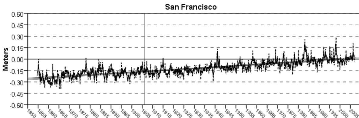
Figure 18. Monthly MSL data for San Francisco after removal of the average seasonal cycle and removal of an apparent datum shift of 0.037 m on September 1897. The total trend is 1.73 +/- 0.13 mm/yr. The time of the April 1906 earthquake is shown by the solid vertical line.
