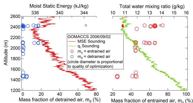
Figure 3. Mass fractions of detrained and entrained air as a function of altitude, along with clear air soundings of MSE and q_t , for 2 September 2006. Larger circles indicate smaller optimization residuals, i.e., less uncertainty in estimated m_d and m_o .
