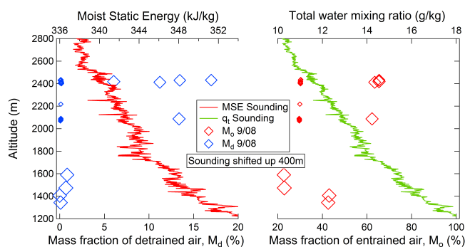
Figure 9. Mass fractions of detrained and entrained air as a function of altitude using shifted clear air soundings of MSE and q_t , for 8 September 2006. Large diamonds indicate smaller optimization residuals, i.e., less uncertainty in estimated m_d and m_o . The soundings used in this case were shifted upwards by 400 m.
