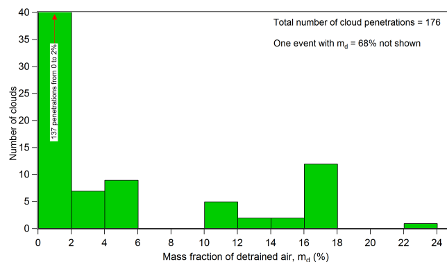
Figure 5. Histogram of detrained air mass fractions for all flight days.
