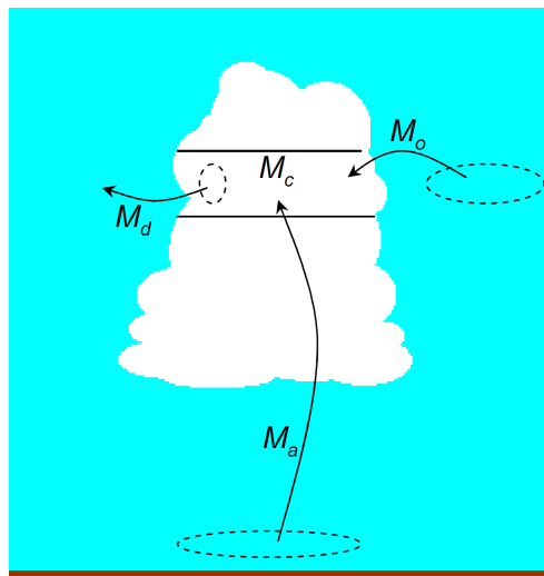
Figure 2. A sketch showing the sources of air that are assumed in this analysis to comprise a cloud. M_a rises adiabatically from cloud base, M_o is entrained laterally at the altitude the cloud is sampled, and M_d is detrained air.
