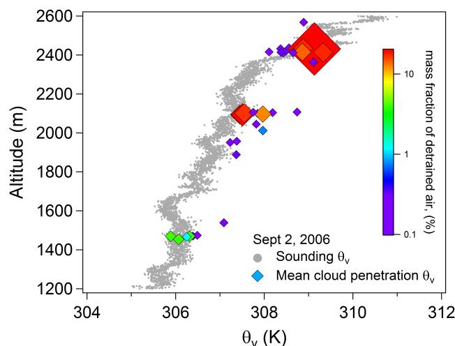
Figure 11. Virtual potential temperature \theta_v of the environmental air (gray dots) from an aircraft sounding and mean \theta_v (colored diamonds) for the air during each cloud penetration on 2 September 2006. The detrainment mass fraction m_d for each penetration is indicated by both color and size of the diamond symbol.
