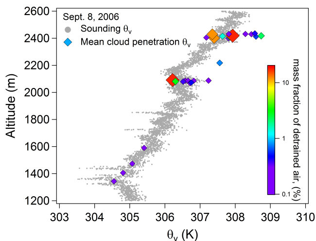
Figure 12. Virtual potential temperature \theta_v of the environmental air (gray dots) from an aircraft sounding and mean \theta_v (colored diamonds) for the air during each cloud penetration on 8 September 2006. The detrainment mass fraction m_d for each penetration is indicated by both color and size of the diamond symbol.
