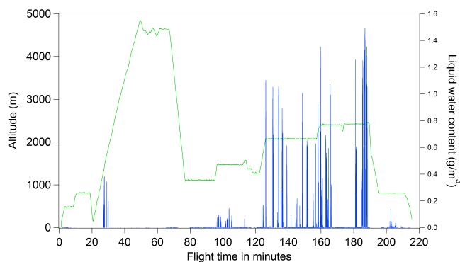
Figure 1. Aircraft altitude and cloud liquid water content as a function of time for the 8 September flight. There were 27 clouds sampled on this day. The clear air sounding occurs from approximately minute 20 to 50.
