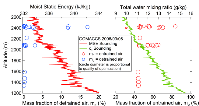
Figure 4. Mass fractions of detrained and entrained air as a function of altitude, along with clear air soundings of MSE and q_t , for 8 September 2006. Larger circles indicate smaller optimization residuals, i.e., less uncertainty in estimated m_d and m_o .
