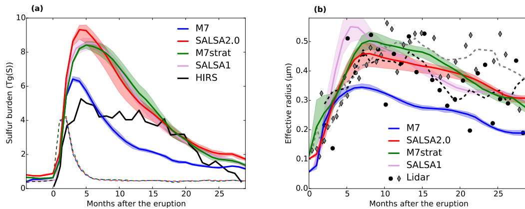
Figure 16. (a) The simulated global burden of SO 2 (dashed curves) and sulfate (solid curves), simulated by SALSA2.0 (red curves), M7 (blue curves), M7strat (green curves), and SALSAl (purple curves). The black curve shows the global sulfate burden retrieved from HIRS observations. (b) The mean effective radius of stratospheric aerosol in the 12 to 20 km layer observed by Raman lidar (diamond markers represent the observations at Laramie, circles represent those at Geesthacht, and dashed lines show the 5-month running means), simulated by SALSA2.0 (red curves), M7 (blue curves), M7strat (green curves), and SALSAl (purple curves). The shading around the solid curves represents the variability of the model ensembles.
