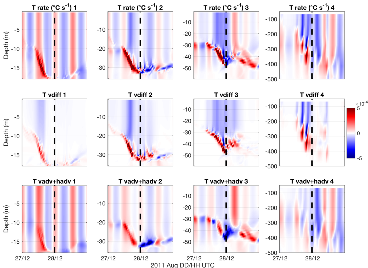
Figure 15. Irene. Temperature diagnostic equation terms at points 1–4 marked in Figure 3 red dots ordered 1–4 northwest to southeast, and in Figure 7 (left), with full temperature rate term at top, vertical diffusion in middle, and vertical + horizontal advection at bottom ( ^{\circ}\text{C s}^{-1} ). Horizontal diffusion is small and thus not plotted. Eye passage marked with vertical dashed line. At point 4, only the top 500 m of the water column is plotted.
