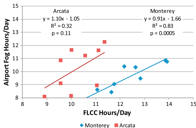
Figure 10. Correlation between airport observations of fog hours and satellite-derived FLCC per day at Arcata and Monterey.
