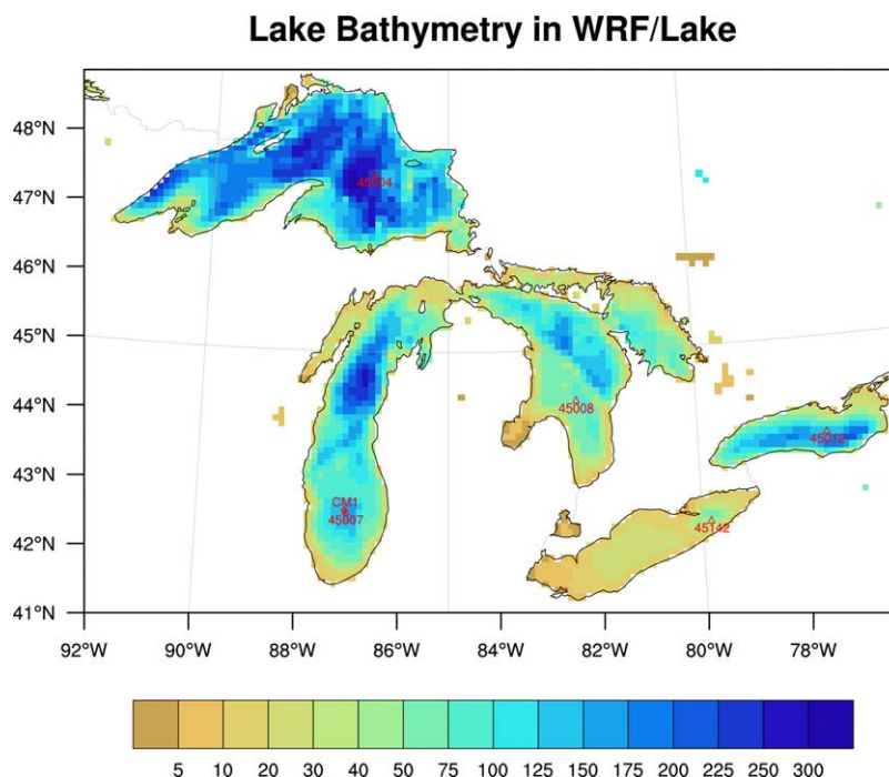
Figure 2. The bathymetry (m) of the Great Lakes in the 1-D Lake model on a 10 km spatial spacing grid. The NOAA National Data Buoy Center (NDBC) buoy stations are marked with triangles. The Mooring station in Lake Michigan is labeled as CM1.
