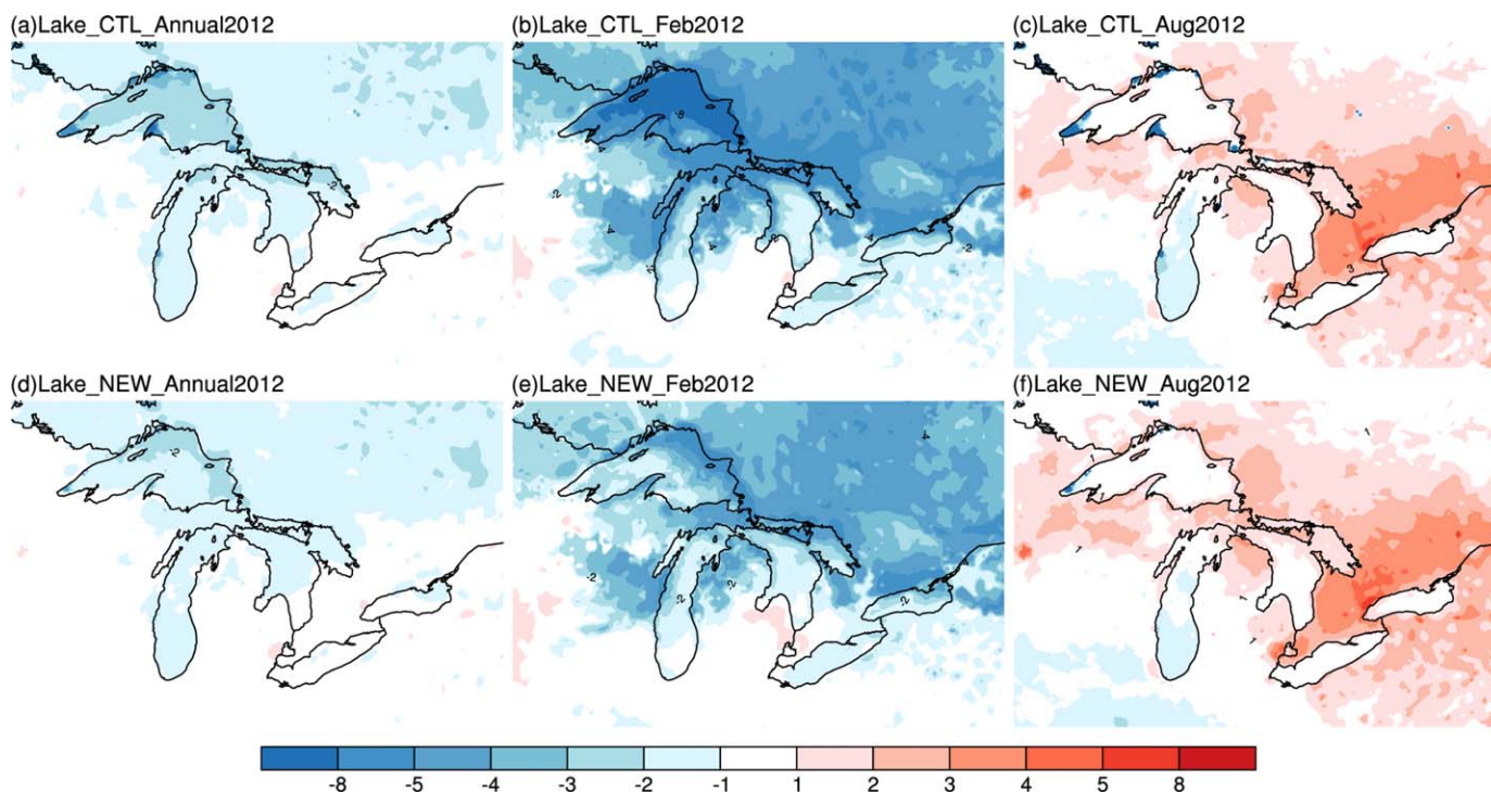
Figure 11. Air temperature ( T_{2m} , °C) differences between the WRF-lake model simulations and NARR reanalysis (model-reanalysis). The 2012 annual T_{2m} are in the left column, the 2012 February mean T_{2m} in the middle column, and the 2012 August mean T_{2m} in the right column.
