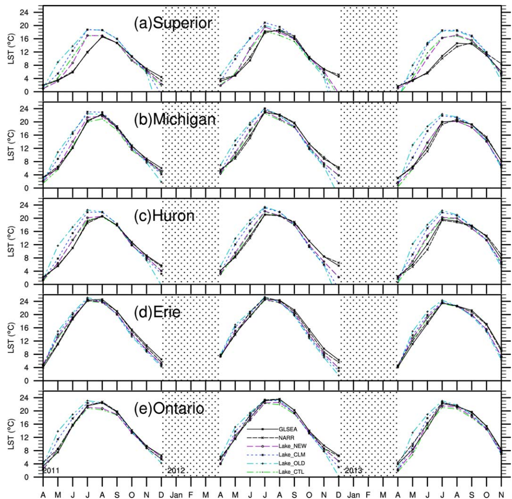
Figure 3. Monthly lake-mean LST (°C) from April 2011 to November 2013 simulated by different lake schemes. The lake surface temperature in the months (December–April) with ice is omitted.
