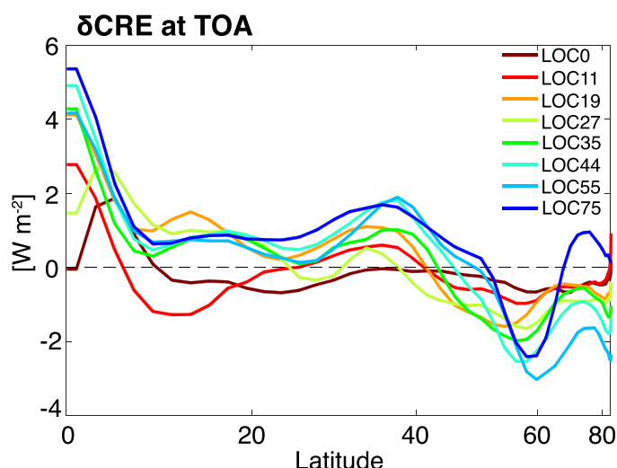
Figure 8. The zonal-mean response of top-of-atmosphere cloud radiative effects for all LOC experiments in FULL.
