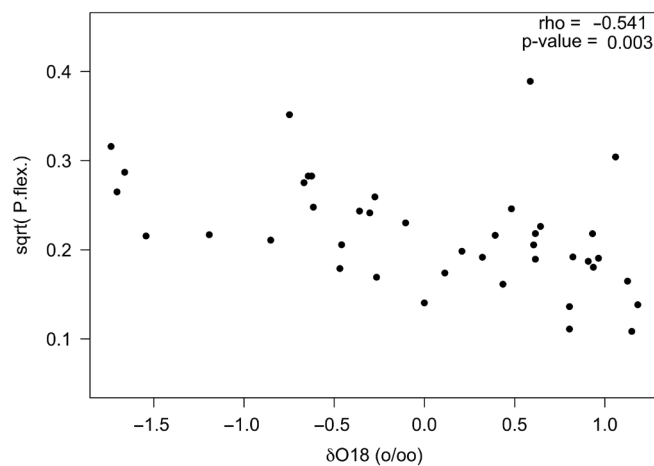
Figure 4. Pinus flexilis / P. albicaulis -type pollen abundance versus median \delta^{18}\text{O} in the 100 yr preceding pollen samples. Pollen abundance is square-root-transformed proportion; \delta^{18}\text{O} units are o/oo Vienna Pee Dee Belemnite carbonate standard (VPDB); P.flex. = Pinus flexilis / P. albicaulis -type; rho = Spearman's rho.
