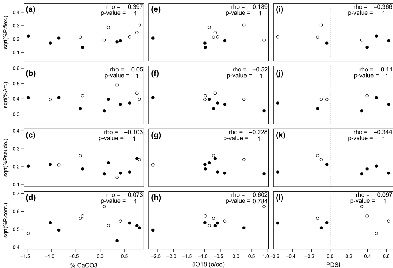
Figure 5. Post-fire pollen abundance versus post-fire climate conditions. Filled points indicate instances when pollen abundance increased from before to after the fire; open points are times when pollen abundance decreased from before to after the fire. \text{CaCO}_3 = calcium carbonate; PDSI = Palmer drought severity index; P.flex. = Pinus flexilis / P. albicaulis -type; Art. = Artemisia ; Pseudo = Pseudotsuga -type; P.cont. = Pinus contorta -type; rho = Spearman's rho. \delta^{18}\text{O} units are o/oo Vienna Pee Dee Belemnite carbonate standard (VPDB). Dashed vertical line in panels (i-l) are PDSI = 0 (normal conditions).
