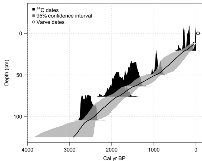
Figure 2. Bayesian age-depth model for Crevice Lake. Gray shading indicates the 95% quantiles for the Bayesian age-depth model, and the thick black line is the 50% quantile. Black distributions show the calendar age probabilities for each radiocarbon date; open circles are varve dates.
