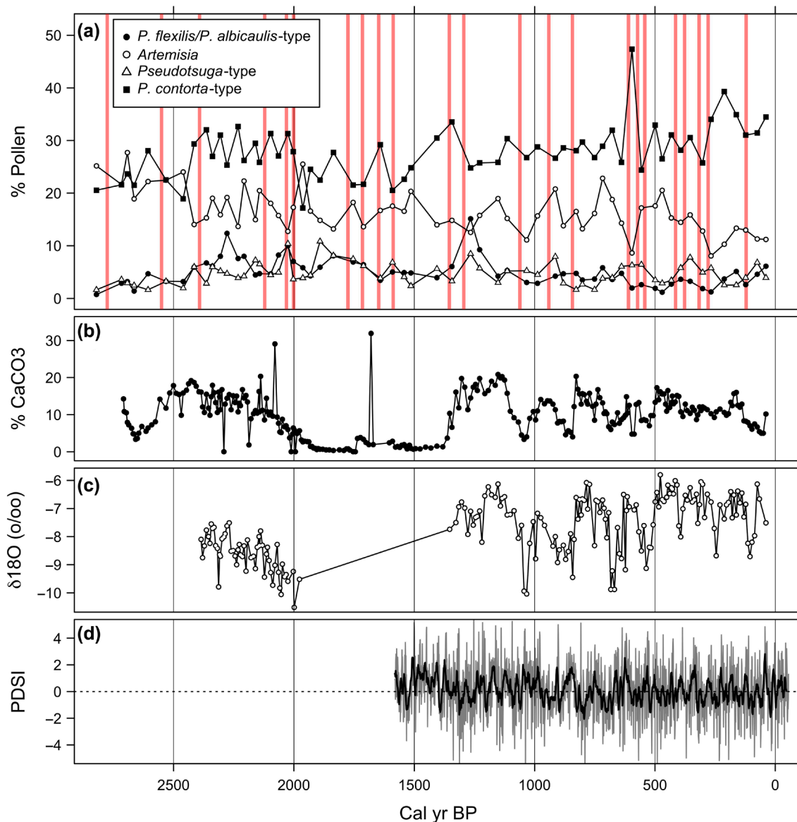
Figure 3. Crevice Lake pollen abundance and climate proxies. (a) Pollen percentages of Pinus flexilis/albicaulis -type (limber pine), Artemisia (sagebrush), Pseudotsuga -type (Douglas-fir) and Pinus contorta -type (lodgepole pine); red vertical lines = fire events inferred from charcoal peaks; (b) % calcium carbonate (CaCO 3 ); (c) δ 18 O (o/oo Vienna Pee Dee Belemnite carbonate standard) (data from Stevens and Dean (2008)); (d) annual (gray line) and 10-yr moving average (black line) Palmer drought severity index (PDSI) (data from Cook et al. (2010)).
