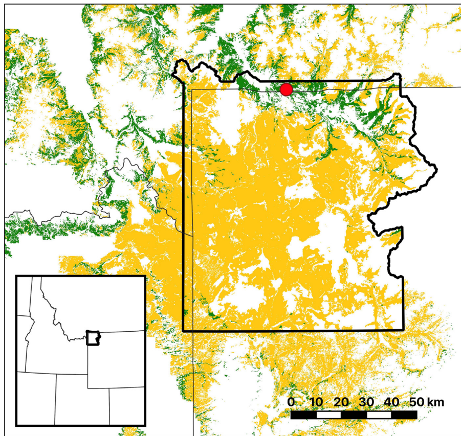
Figure 1. Map of the study region. Red point = Crevice Lake; yellow shading = regions dominated by lodgepole-pine; green shading = regions dominated by Douglas-fir; thick black line = border of Yellowstone National Park.
