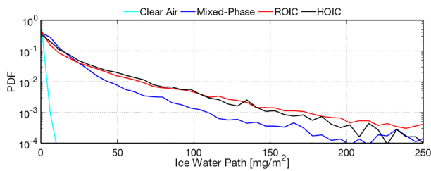
Figure 4. Univariate PDF of the IWP for all clouds observed with IR OD < 1.5. All possible IWP data is presented that has a valid refined CSCI identification.
