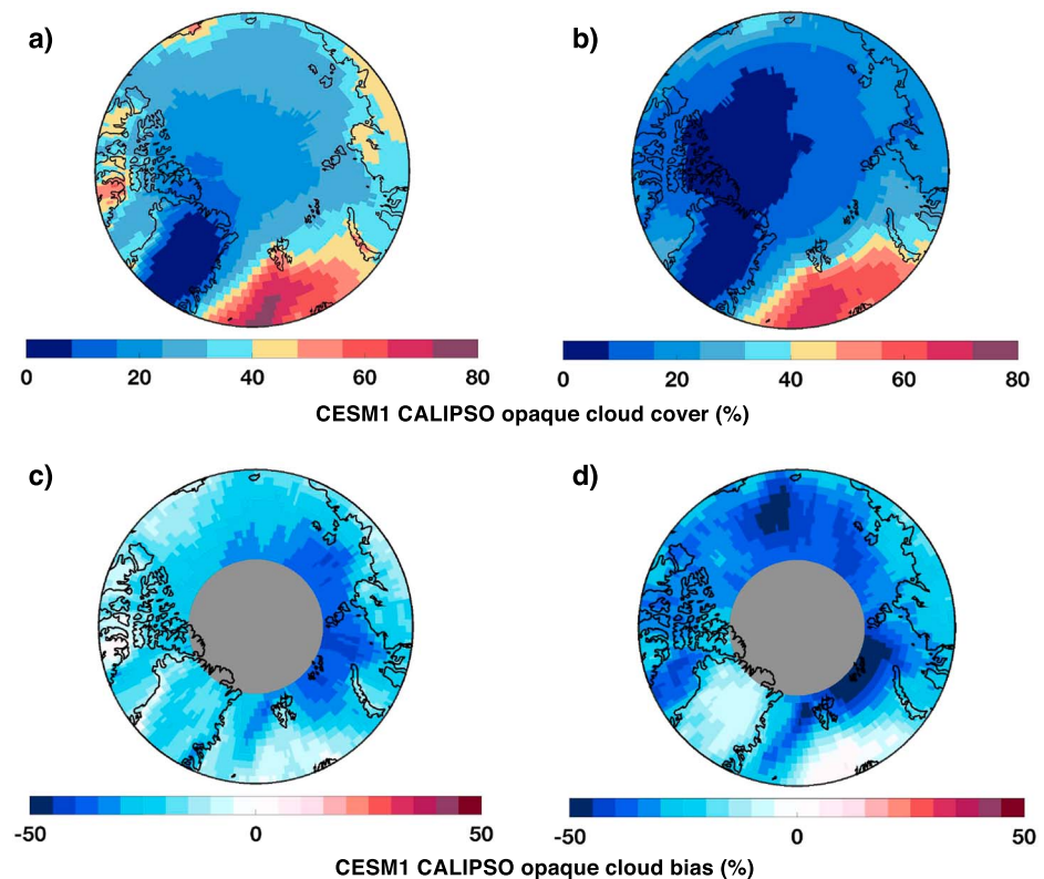
Figure 3. Mean state from 2006 to 2015 for CESM1 CALIPSO opaque cloud cover during (a) summer (JJA) and (b) fall (SON), and difference between observed and simulated CESM1 CALIPSO opaque cloud cover during (c) summer (JJA) and (d) fall (SON). CESM1 CALIPSO opaque cloud biases are calculated against CALIPSO-GOCCP observations.
