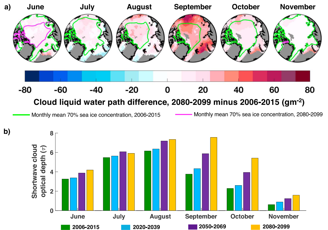
Figure 7. (a) Difference in CESM1 monthly cloud liquid water path between 2006–2015 and 2080–2099. The green (pink) line is the 70% monthly mean sea ice concentration for 2006–2015 (2080–2099). (b) Time series of monthly mean summer (JJA) and fall (SON) CESM1 shortwave cloud optical depth within the intermittent mask for 2006–2015 (green), 2020–2039 (blue), 2050–2069 (purple), and 2080–2099 (yellow).
