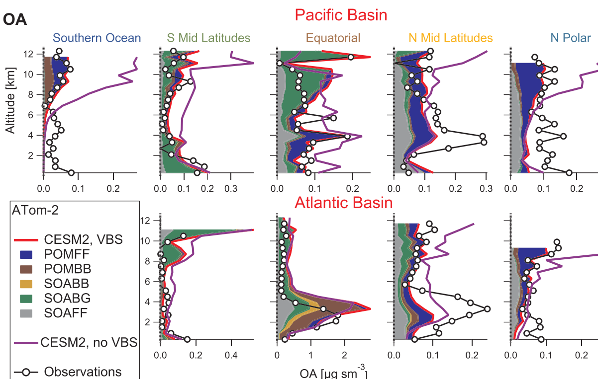
Figure 9. As in Figure 12, but for ATom 2 instead.
