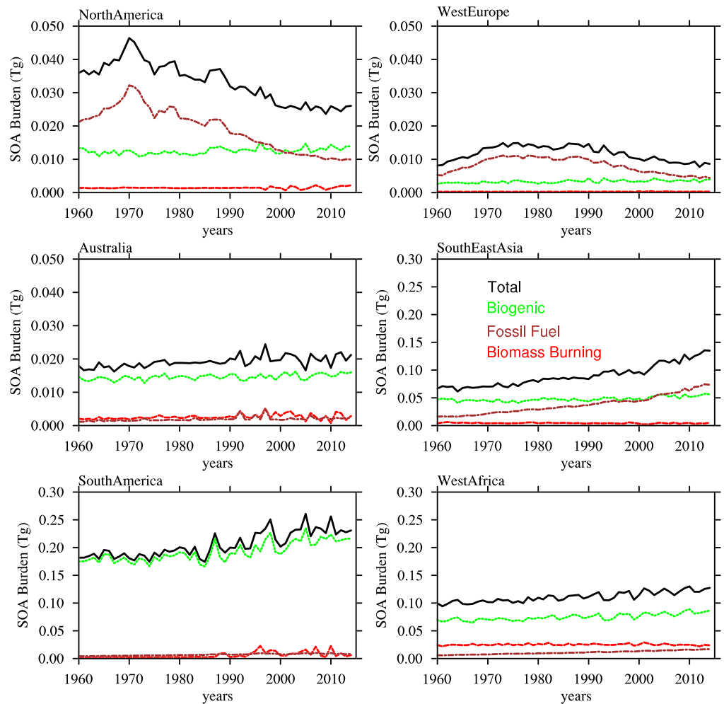
Figure 13. Annually averaged total SOA burden (black), and SOA burden from separate precursor sources, including biogenic (green), fossil fuel (brown), and biomass burning (red), averaged over six regions as indicated in Figure 8, between 1960 and 2014 derived using WACCM6-VBSext.
