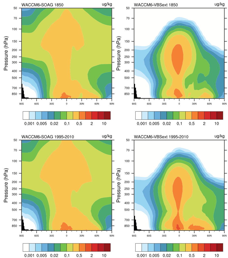
Figure 2. Secondary (SOA) zonal and annual mean distribution for WACCM6-SOAG (left) and WACCM6-VBSext (right), averaged over 10 years for preindustrial conditions (top) and between 1995 and 2010 (bottom).
