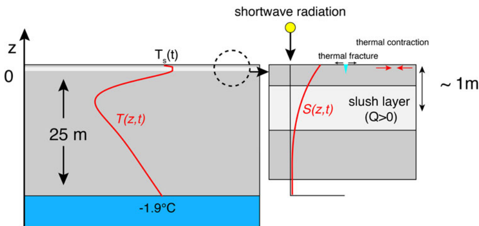
Fig. 8. Schematic depiction of 1-D model domain used for simple thermal modeling. The temperature- depth profile T(z, t) (left side of figure) represents conditions around \sim 1 January when solar absorption below the surface generates a subsurface meltwater/slush layer. The schematic depiction of solar heating S(z, t) (right side of figure) displays exponential decay with depth below the surface with a skin depth, d , of 0.5 m, which is taken from observations by Jarvinen and Leppäranta (2013).
