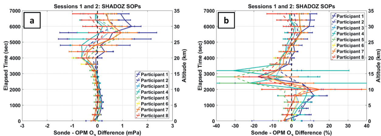
FIG. 6. (a) Participant mean profiles relative to OPM in partial pressure (mPa) and (b) percentage deviation (sonde minus OPM/OPM). Based on five simulations per participant.
