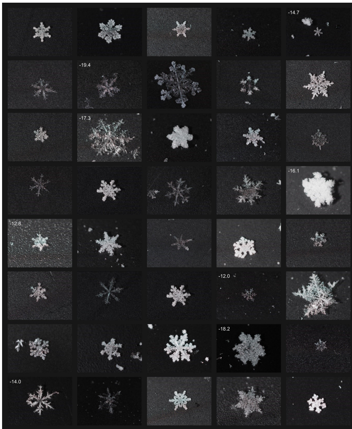
Figure S3. Examples of images of the analysed dendrites taken by macro (1:1) photography. Crystals of which the residues immersed in a water droplet froze above -20\text{ }^{\circ}\text{C} have the freezing temperature added in the upper left corner of their image. Each image shows an area of 8.6\text{ mm} \times 6.4 on the black surface where the crystals had been collected.
