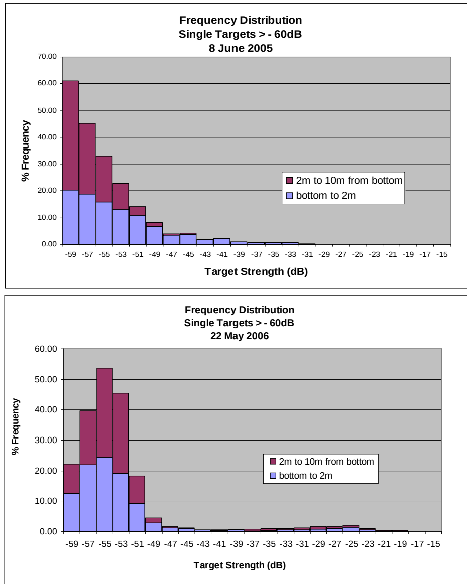
Figure 9. Frequency distribution of single targets > -60\text{dB} . The water column is divided into two regions: 0-2m from the bottom and 2-10m from the bottom.
