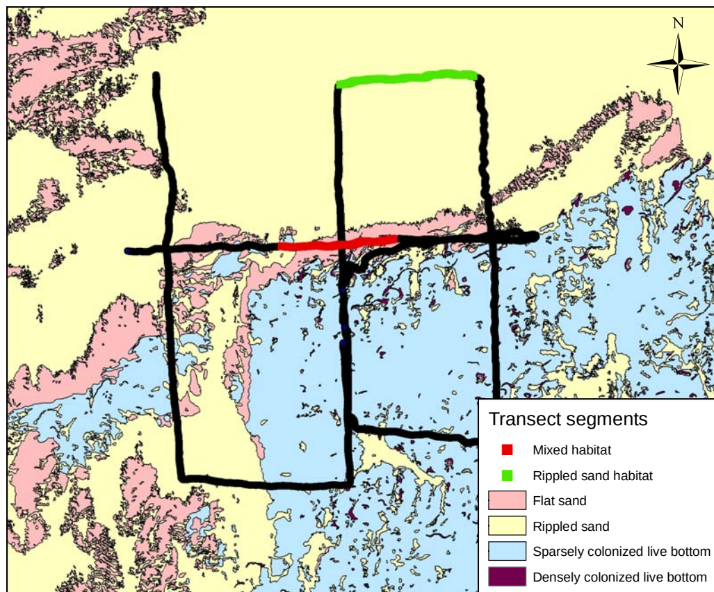
Figure 11. Location of two segments of the May 22, 2006 acoustic transect with different benthic habitat types.
