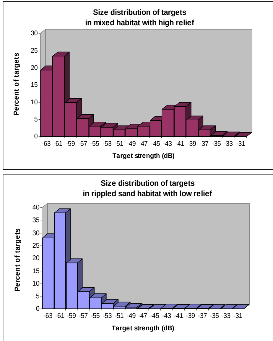
Figure 12. Distribution of target strength (as an indicator of fish size) in water regions above mixed habitat with high relief (upper graph) and rippled sand habitat with low relief (lower graph). Targets in the mixed relief habitat show a bimodal distribution compared to the sand habitat. The sand habitat has a higher percentage of smaller organisms.
