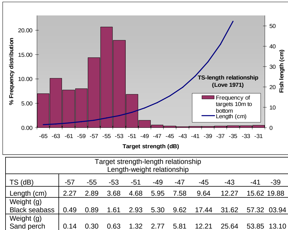
Figure 10. Target strength frequency distribution (May 2006) with TS-fish length model [ TS = 19.1 \log L + 0.9 \log \lambda - 23.9 where L =length (cm) and \lambda is frequency (Love 1971)]. Length-weight relationship W = a L^b for black seabass ( Centropristis striata ) where a=0.0649 and b = 2.468 (Bohnsack and Harper 1988) and sand perch ( Diplectrum formosum ) where a= 0.0114 and b = 3.078 (fishbase.org).
