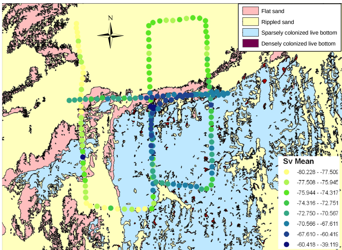
Figure 13. Map of S_{v\_mean} (indicator of fish biomass) from May 2006 acoustic survey in relation to benthic habitats.
