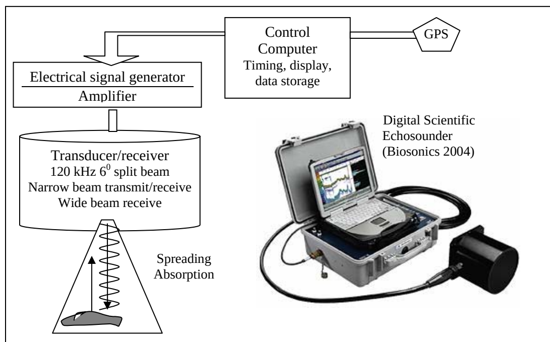
Figure 3. Basic architecture and components of a scientific fisheries acoustics system. A typical split-beam fisheries acoustics system includes a signal generator that creates the electrical signal or ping. A transducer transmits a sound pressure wave through the water column. The transducer also captures the backscatter signal in the form of sound pressure and converts it back to an electrical signal reported as volume backscattering strength in decibels. A deck side computer controls the timing of the electrical signal, data acquisition, data display, and GPS input. In a split-beam system, the beam is divided into quadrants, allowing for the location of the target within the beam to be determined and a target strength correction applied to compensate for off-axis loss of the reflected sound.
