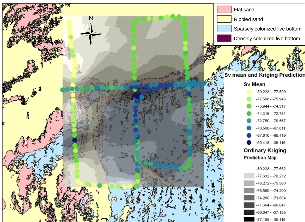
Figure 14. Interpolation of S_{v\_mean} to predict distribution of fish biomass in unsampled locations (Mean prediction error = -0.0076; RSME standardized = 1.048).
