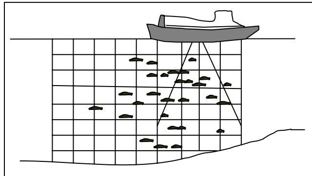
Figure 2. Underwater acoustics data collection provides fine resolution mapping of the water column. As the ship travels along a transect, a signal is sent into the water column. The strength of the returned signal and the time of travel are recorded to estimate the size and depth of the target.
