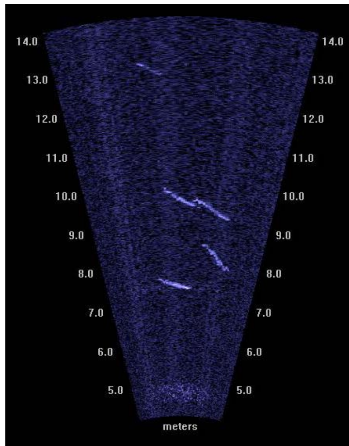
Figure 15. High resolution image (1.8mHz) taken with a DIDSON unit along the May 2006 survey track. Scale indicates distance from lens extending out horizontally.
