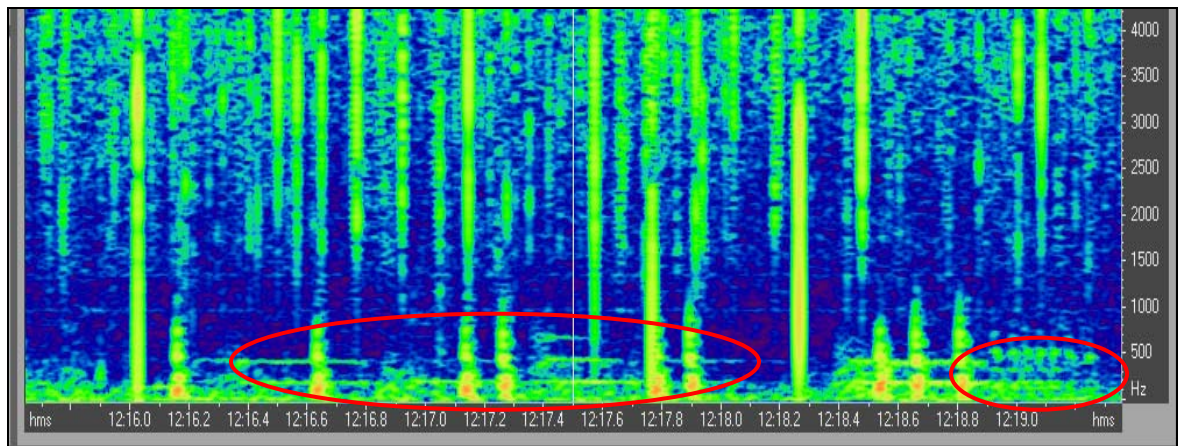
Figure 16. Spectral frequency of sounds collected using underwater passive acoustic recording devices at GRNMS during the May 2006 survey. Fish sounds recorded here include toadfish (large circle) mixed with a purring sound (small circle). These sounds range in frequency from 10 to 1200Hz.
