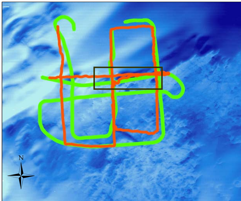
Figure 7. Relief map of GRNMS overlaid with acoustic survey tracks conducted in the late afternoon on 8 June 2005 (green) and during the evening on 22 May 2006 (red). The black rectangle indicates a region of high relief.
