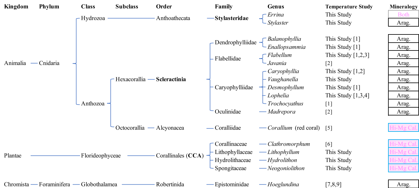
[1]Case et al., 2010, [2]Cuny-Guiriec, et al 2019, [3]Montagna et al., 2014, [4]Raddatz et al., 2013, [5]Chaabane et al., 2019, [6]Anagnostou et al., 2019, [7]Hall & Chan 2004, [8]Bryan & Marchitto 2008, [9]Marchitto et al., 2018
