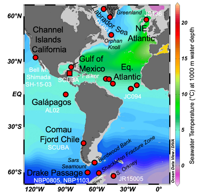
Fig. 3. Location of modern coral (circles) and coralline algae (square) samples used in this study with respective cruise identifiers (white text). Base map shows World Ocean Atlas gridded seawater temperature at 1000 m (Locarnini et al., 2013).
