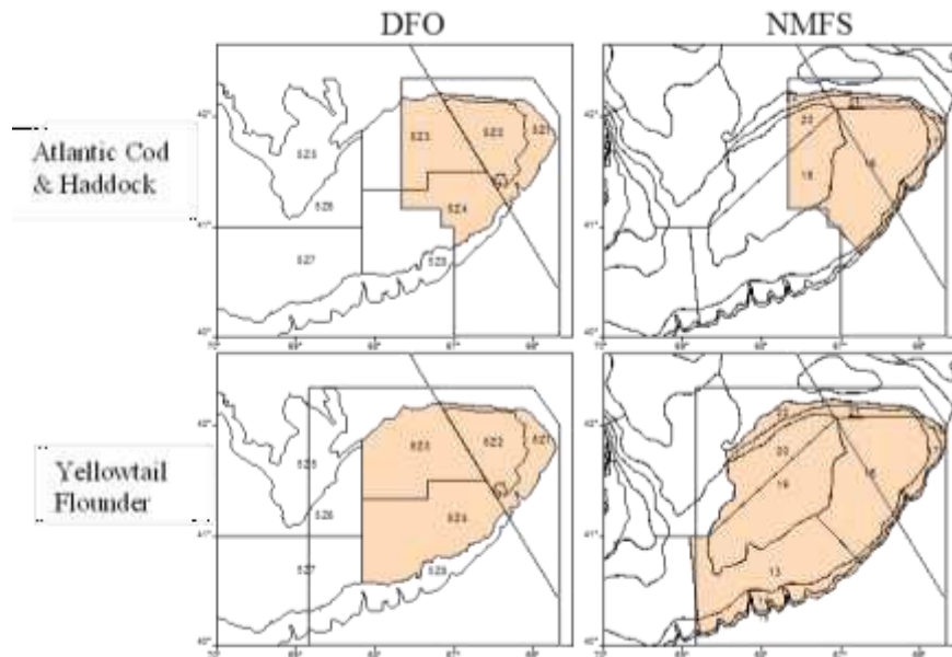
Figure 1. The management areas for Atlantic Cod, Haddock (upper panel), and Yellowtail Flounder (lower panel) on Georges Bank (thick grey line), including the Canada/USA boundary line (thin grey line) across which resource distribution was determined.
