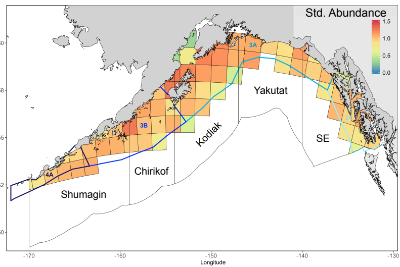
standardized by predicted mean
