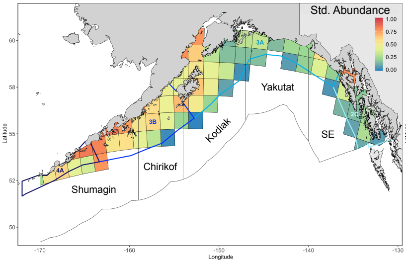
standardized by predicted max
