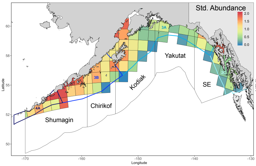
standardized by predicted median
