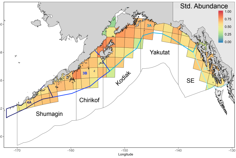
standardized by predicted max
