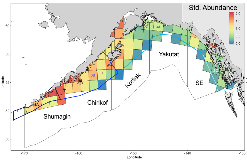
standardized by predicted mean
