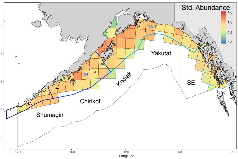
standardized by predicted median
