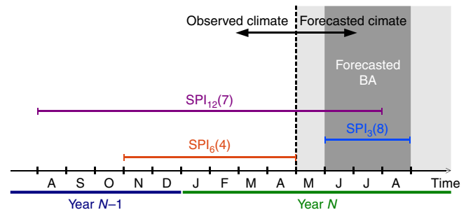
Fig. 1 Schematic view of the proposed burned area forecast system. In order to forecast burned area (BA) in JJA of year N (dark grey shadow), we rely on the climate forecast issued on May of the same year (dashed line). Before May, we have the observed climate data, while from May on (light grey) we only have seasonal climate forecasts. Observations and forecasts can be merged to construct the SPI_t(M-m) –BA model, depending on the values of the parameters t (which can take a value of 3, 6 or 12 months) and M-m (which, in the illustrated example, can vary between March and August of year N , i.e. from the last month of the season being forecasted, back to the prior 6 months). As examples, we represent how climate observations and forecasts should be merged to compute SPI_{12}(7) (purple line); how SPI_3(8) is constructed from climate forecasts only (light blue line); and how SPI_6(4) (orange line) is computed only from observations
